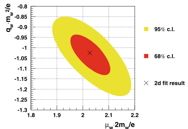
Fig. 12 The log-likelihood contours for a two-parameter fit to q_W and \mu_W , respectively the electric quadrupole and magnetic dipole moments of the W^+ boson, obtained from the simultaneous fit to \lambda_\gamma and \Delta\kappa_\gamma . Results from the semi-leptonic, fully hadronic and single W final states have been combined in the plot, and contributions from both statistical and systematic effects are included. The Standard Model expectations for the quantities plotted are: q_W m_W^2/e = -1 and \mu_W 2m_W/e = 2
