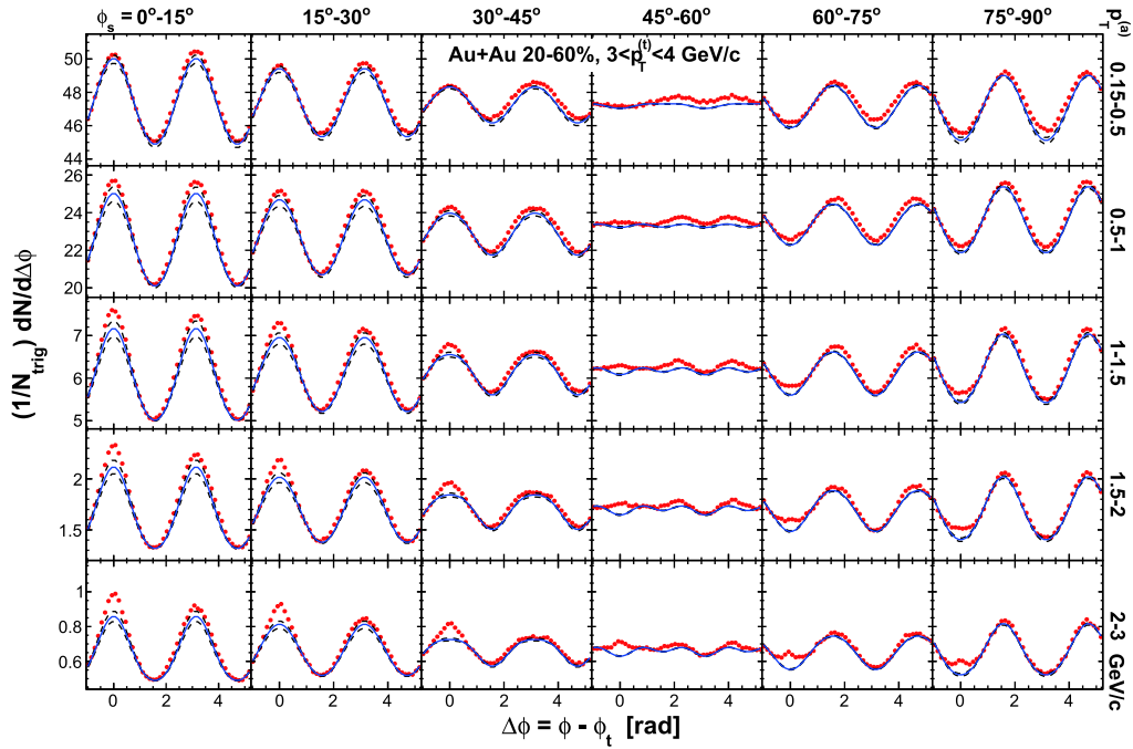
Fig. C1. (color online) Raw dihadron \Delta\phi correlations with trigger particles in six slices of azimuthal angle relative to the event plane, \phi_s = |\phi_t - \psi_{\text{EP}}| . The data are from minimum-bias 20%-60% Au+Au collisions. The trigger p_T range is 3 < p_T^{\text{trig}} < 4 GeV/c. Five associated particle p_T^{(a)} bins are shown. Both the trigger and associated particles are restricted within |\eta| < 1 . The triangle two-particle \Delta\eta acceptance is not corrected. Statistical errors are smaller than the symbol size. The curves are flow modulated ZYAM background including v_2 and v_4\{\psi_2\} by Eq. (1). The used v_2 values are given in Table 1 from four-particle v_2\{4\} and two-particle v_2\{2, \eta_{\text{gap}} = 0.7\} (dashed curves) and the average v_2 from the two methods (solid curve). The v_4\{\psi_2\} is taken from the parameterization in Eq. (15).
