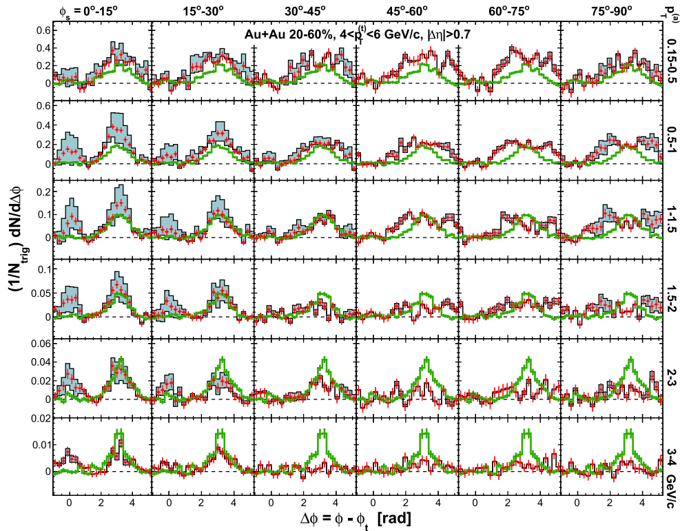
Fig. C12. (color online) Same as in Fig. C11 but but for trigger particle 4 < p_T^{(t)} < 6 GeV/c and six bins in associated particle p_T^{(a)} .
