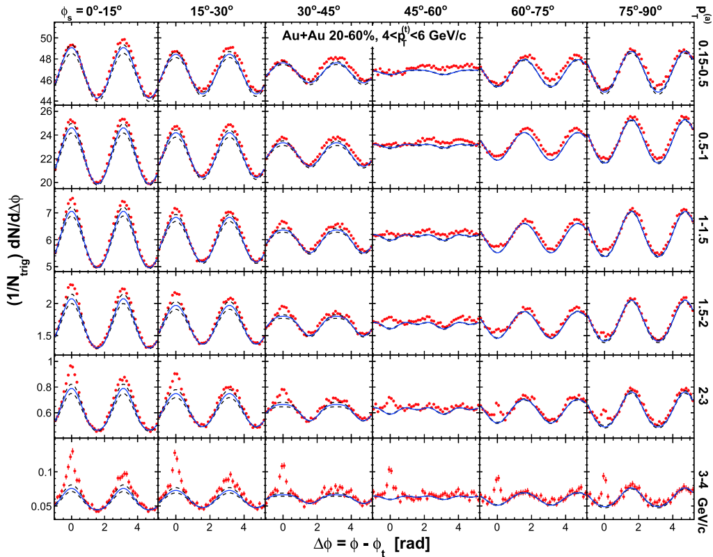
Fig. C2. (color online) Same as in Fig. C1 but for trigger particle 4 < p_T^{\text{trig}} < 6 GeV/c and six bins in associated particle p_T^{(a)} .
