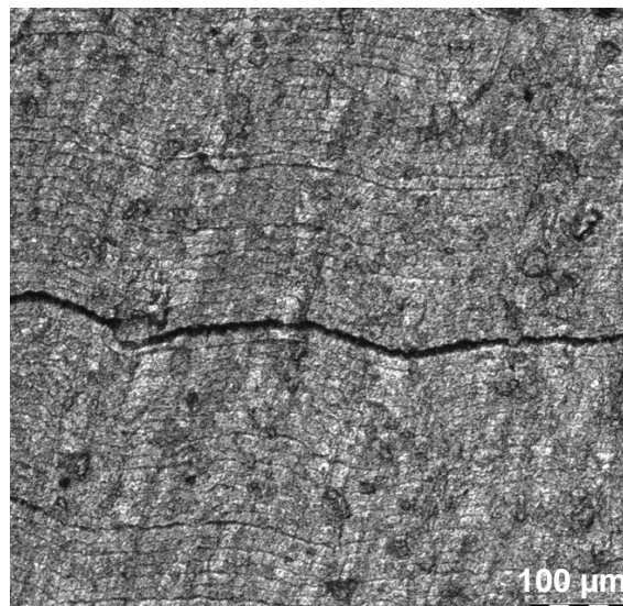
Figure 5 A surface of the stack of foils with visible gaps between individual layers
