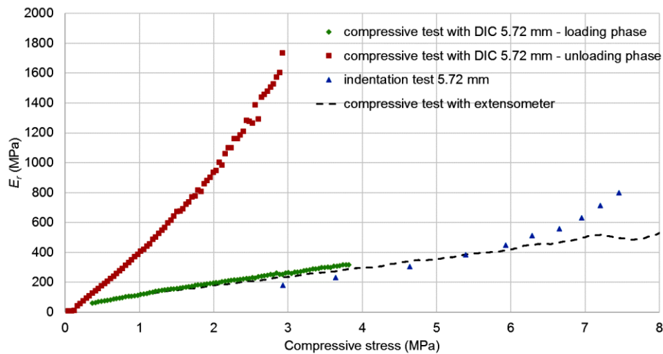
Figure 7 A comparison of measurements of effective modulus using compression test with DIC and video extensometer and indentation method with stack size 5.72 mm was used for DIC and indentation method
