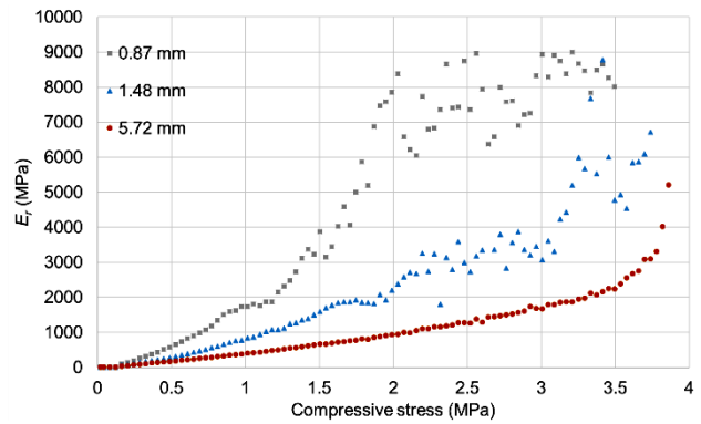
Figure 4 A relationship between effective modulus and compressive stress for unloading phase of the compression test with tested stack thicknesses 0.87, 1.48 and 5.72 mm
