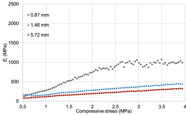
Figure 3 A relationship between effective modulus and compressive stress for loading phase of the compression test with tested stack thicknesses 0.87, 1.48 and 5.72 mm
