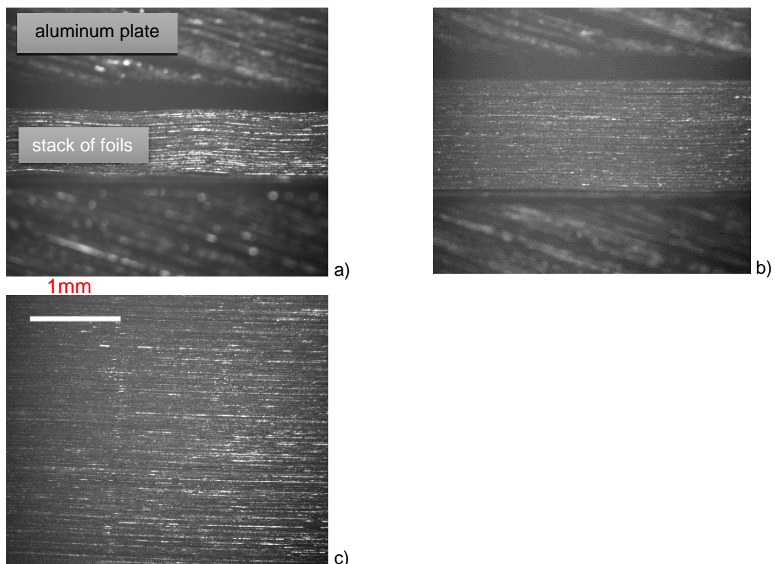
Figure 1 Images from the FLIR camera for thicknesses of stack of foils of a) 0.87 mm, b) 1.48 mm, c) 5.72 mm
