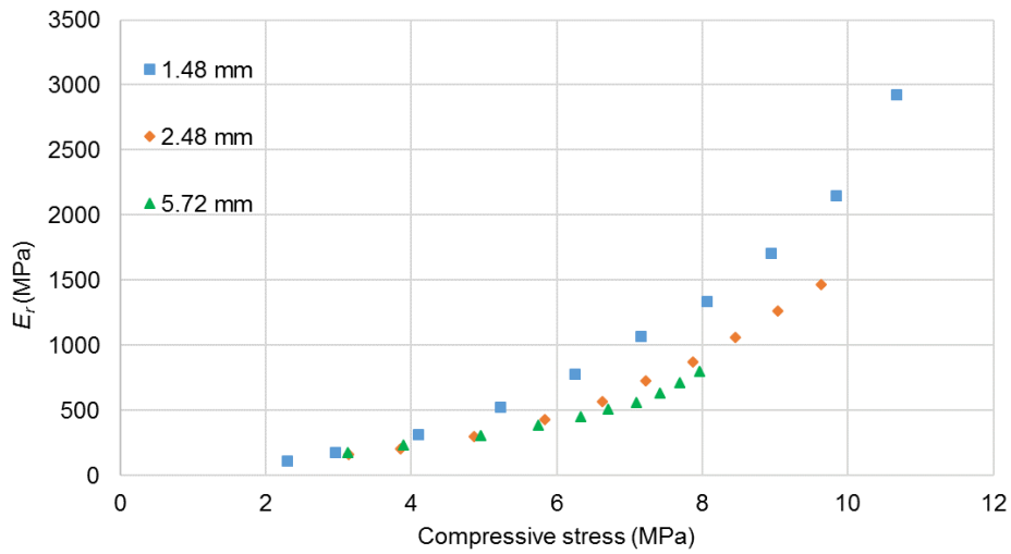
Figure 6 A relationship between effective modulus and compressive stress of the indentation test with tested stack thicknesses 1.48, 2.48 and 5.72 mm
