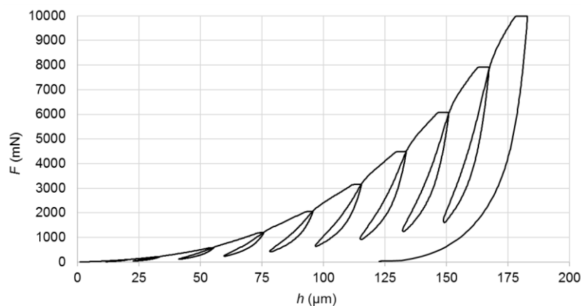
Figure 2 F - h curve of CMC indentation of stack of foils with thickness 2.48 mm
