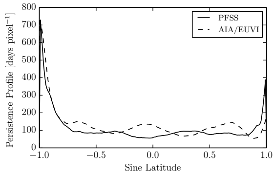
FIG. 12.— Coronal hole persistence map projected as a function of latitude. The two profiles are in units of days\ pixel^{-1} . The PFSS model calculates a further extension of open field persistence from the poles as compared with our AIA/EUVI observations. The persistence value at low latitudes agrees in value, but with variations in distribution visible in Figure 11.
