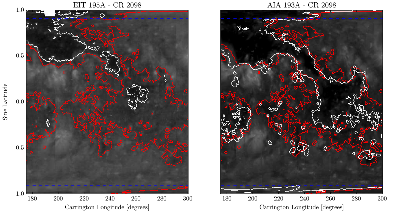
Fig. 5.— Left: EUV synoptic image from EIT 195 Å, with contours of calculated coronal hole boundaries from EIT data in white and AIA data in red. Right: EUV synoptic image from AIA 193 Å, with contours of calculated coronal hole boundaries from AIA data in red, and EUVI A/B data in white. The enhanced contrast of the AIA instrument is immediately apparent for the calculation of coronal hole boundaries.
