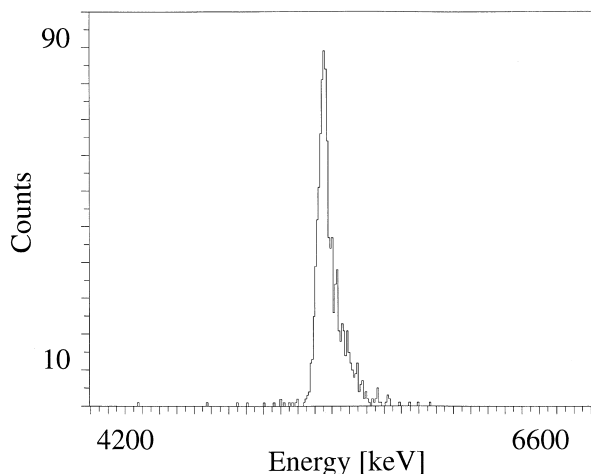
Fig. 6. Spectrum in the ^{210}\text{Po} \alpha decay region obtained with the bolometer with the Johnson and Mathey absorber.
