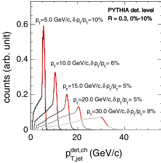
FIG. 3. Distribution of jets with R = 0.3 in p + p collisions at \sqrt{s} = 200 GeV, generated by PYTHIA: p_{T,jet}^{det} (detector level) for fixed values of p_{T,jet}^{part} (particle level). Detector-level effects are for the environment of central Au + Au collisions. The red lines are Gaussian fits to the narrow peak, with relative width given as \delta p_T/p_T .
