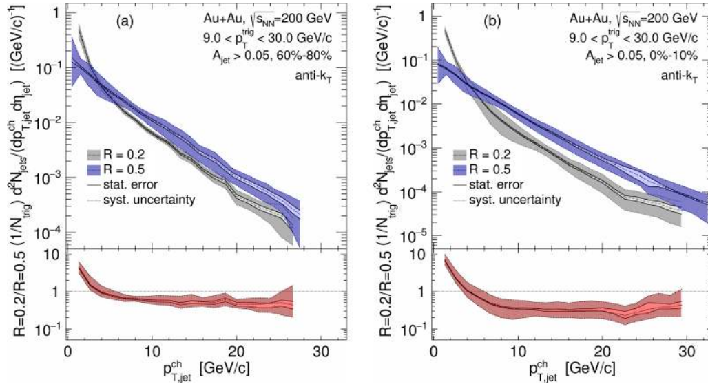
FIG. 20. Distributions of Y(p_{T,jet}^{ch}) for R = 0.2 and 0.5 (upper subpanels) and their ratios (lower subpanels) in peripheral (a) and central (b) Au + Au collisions at \sqrt{s_{NN}} = 200 GeV.
