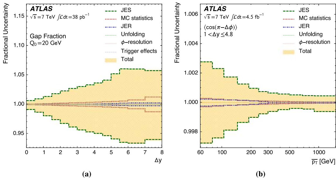
Fig. 2 Summary of systematic uncertainties on a the gap fraction as a function of \Delta y and b the \langle \cos(\pi - \Delta\phi) \rangle distribution as a function of \overline{p_T} . Here the systematic uncertainties from the jet energy scale ( dark dashes ), Monte Carlo statistical precision ( dark dots ), jet energy res-
