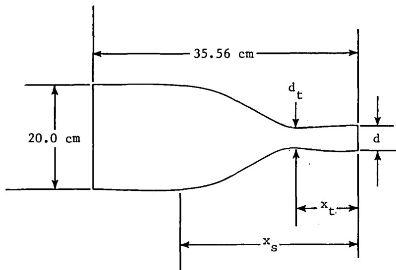
Contoured nozzle
