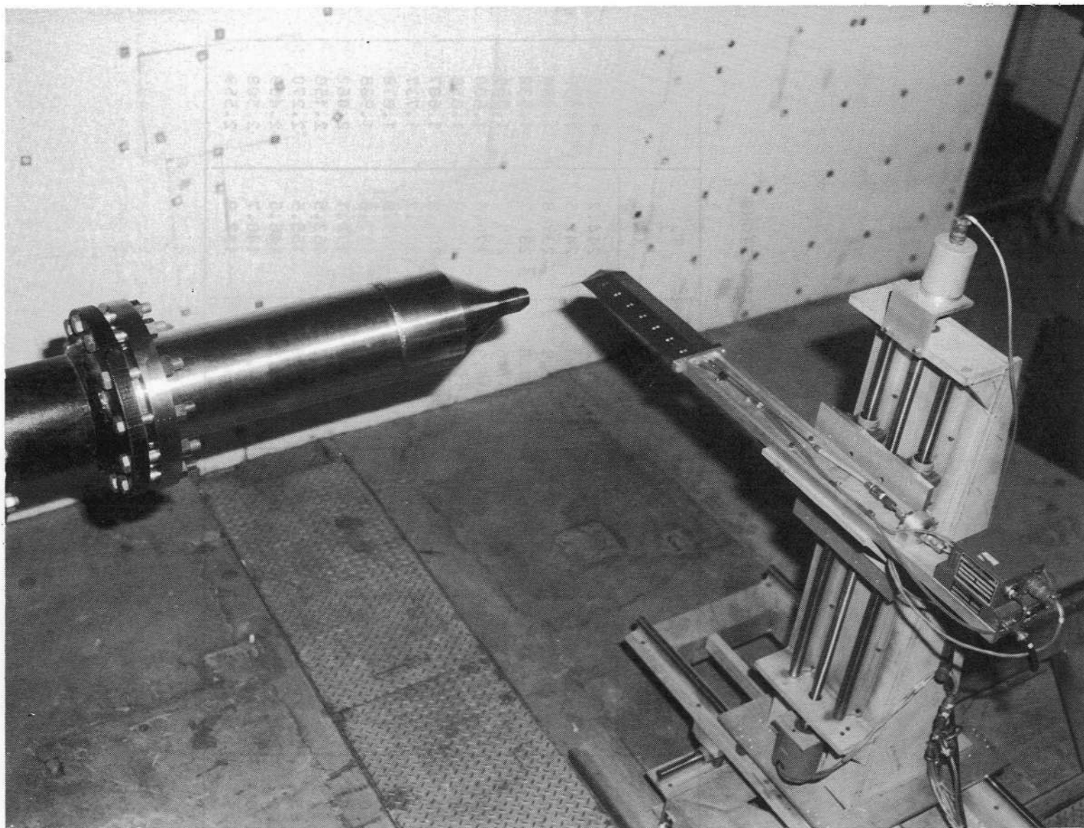
Figure 1.- Nozzle and pressure probe drive mechanism in Langley Jet Noise Laboratory.
