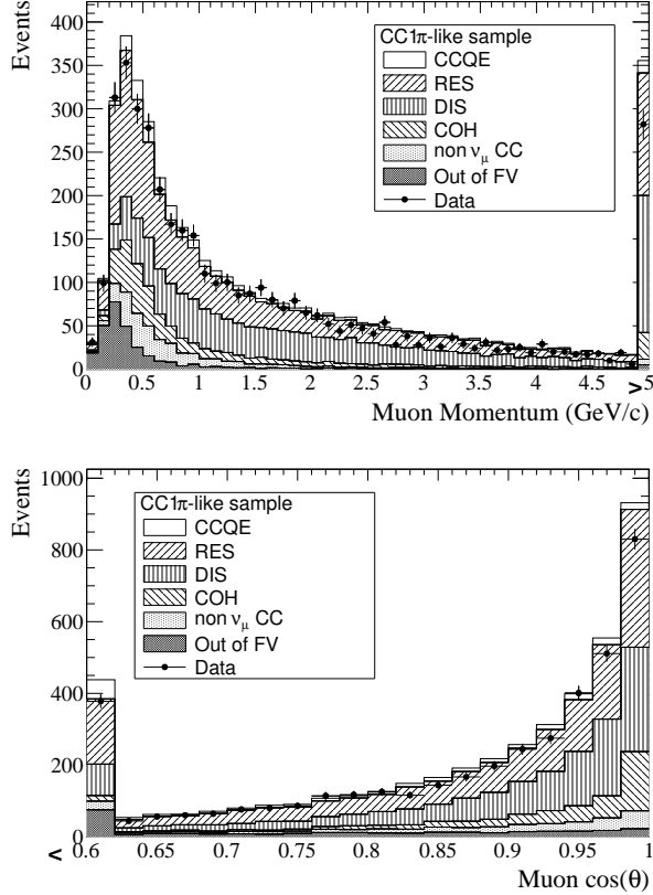
FIG. 11: Muon momentum and angle distribution for the \text{CC}1\pi^+ -like sample. These are compared to the simulation, broken down into the different reaction types, with all systematic parameters set to their nominal values.
