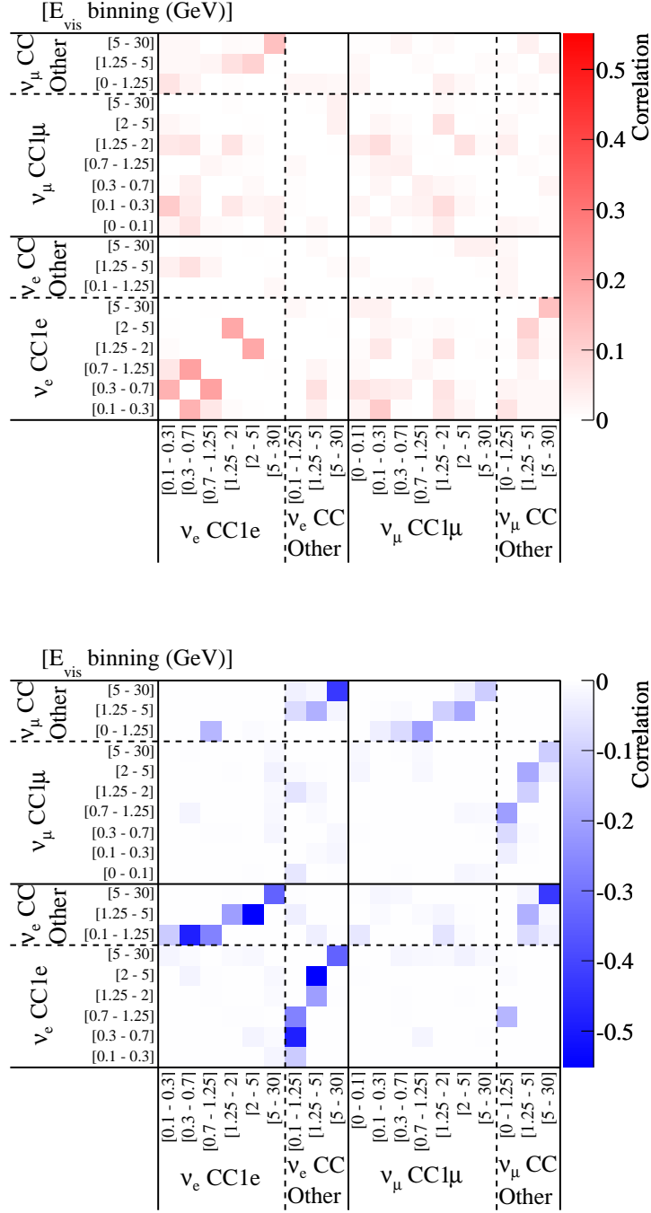
FIG. 24: The correlations between the estimated efficiencies for the final state topologies CC 1e and CC e other for the \nu_e CC event selection and CC 1\mu and CC \mu other for the \nu_\mu CC event selection. The upper figure shows the combinations with positive correlation, and the lower with negative correlation. The diagonal correlations (correlation = 1) are not shown.
