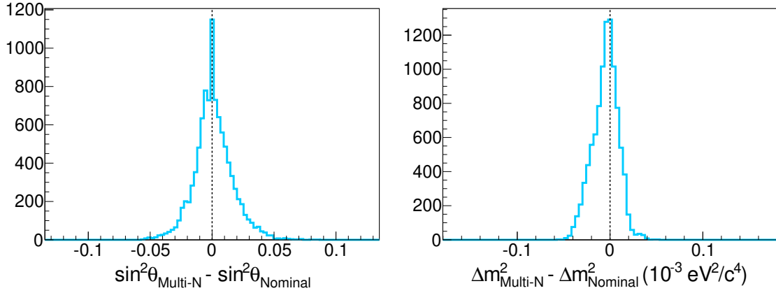
FIG. 30: Difference in the point estimates of \sin^2\theta_{23} (left) and |\Delta m^2| (right) between pairs of toy MC datasets with and without including multi-nucleon effects.
