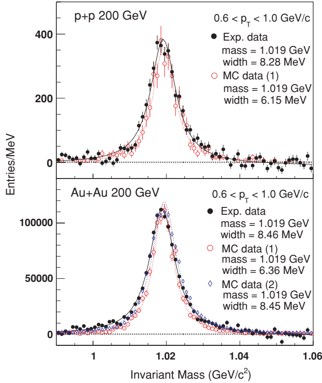
FIG. 9. (Color online) Invariant mass distributions of \phi meson at 0.6 < p_T < 1.0 \text{GeV}/c in p + p 200 GeV (NSD) and Au + Au 200 GeV (0–5%) collisions. Solid symbols: experimental data. Open symbols: MC simulation. Curves are the results of a Breit-Wigner function fit. Note: Two sets of MC data are shown for Au + Au 200 GeV, and see text for details.
