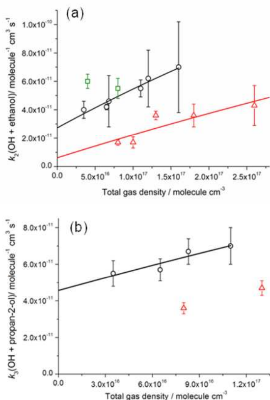
Figure 4. (a) Pressure dependence of the rate coefficient for OH + ethanol at 54-56 K (green open squares, Ar bath gas), 82-89 K (black open circles, \text{N}_2 bath gas) and 133-148 K (red open triangles \text{N}_2 bath gas). All values of the temperatures, densities and rate coefficients are given in Table 1. The black and red lines are the extended Lindemann-Hinshelwood fits (E8) to the data at 82-89 K and 133-148 K respectively. See text for details. Error bars represent propagation of the 95 % confidence limits (including the whole covariance matrix) in the bimolecular rate coefficients with the errors in the expansion densities. (b) Pressure dependence of the rate coefficient for OH + propan-2-ol at 89 K (black open circles) and 133-138 K (red open triangles). The black line is the extended Lindemann-Hinshelwood fit (E8) to the data at 89 K. Error bars as for (a).
