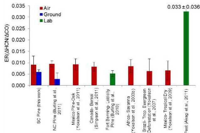
Fig. 10. Comparison of \Delta HCN/\Delta CO study-average emission ratios (mol/mol) measured from airborne (red), ground-based (blue), and laboratory (green) platforms from five North American pine-forest fuels (leftmost bars). We also show four ER(\Delta HCN/\Delta CO) in other fuel types for comparison. Error bars ( 1-\sigma ) are included for all data. The large variation shown for peat is due to a very large value for Indonesian peat that is included in the calculation.
