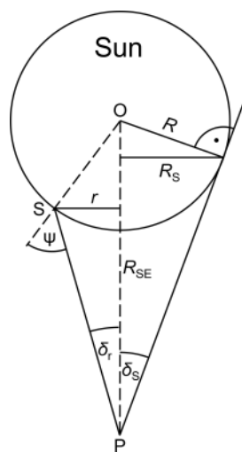
Figure 6. Limb darkening geometry. The Sun is centered at point O and has the radius R . The observer is at point P at a distance R_{SE} from the center of the Sun and is looking at point S on the surface of the Sun. From the point of view of the observer, S is at an angle \delta_r relative to the center of the Sun, and the Sun's limb is at angle \delta_s . The angular radius of the solar disk as viewed by the observer is R_S , and the angular radius associated with S is r . \psi is the angle between the Sun's normal at S and the line between S and P.
