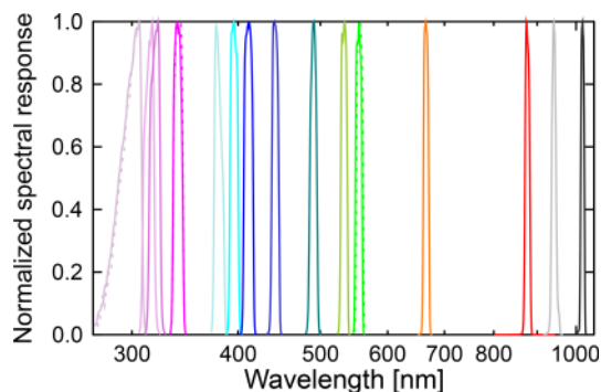
Figure 3. Normalized spectral response functions of the GUVIS-3511 radiometer discussed in this study. Functions were measured with BSI's spectral tester (Bernhard et al., 2005a) and corrected for the finite bandpass of the tester using a simple deconvolution routine also described by Bernhard et al. (2005a). Color coding is identical to that in Fig. 8. Note that the x axis is logarithmic to emphasize the UV range. A version of the figure, plotted separately for UV, visible, and IR wavelengths, is part of the Supplement.
