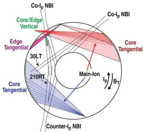
FIG. 1. Top-down view of the DIII-D tokamak displaying three neutral beam lines and CER sightlines. Viewchords of carbon (shaded) and main-ion (lines) system core viewchords indicated viewing co- I_p and counter- I_p neutral beams.
