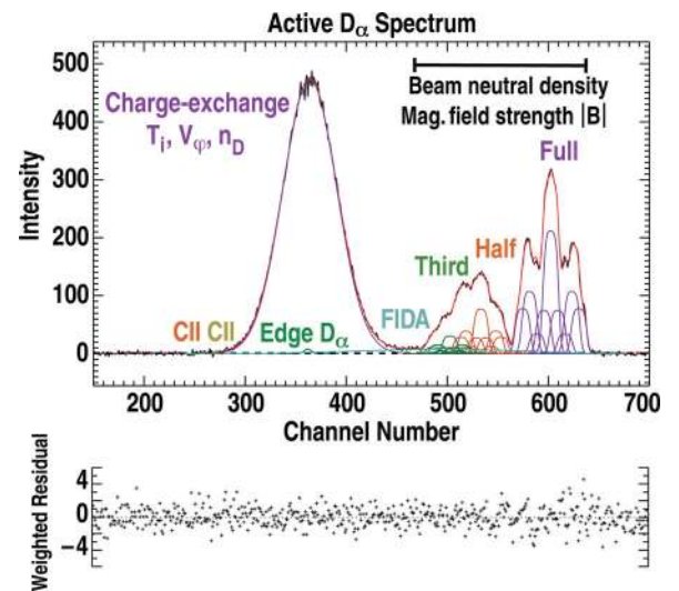
FIG. 2. Complete fit to active D_\alpha spectrum obtained by timeslice subtraction. The fit model incorporates the thermal charge-exchange feature localized between channels 280–450, beam emission of 81 \text{ keV} injection identified as full, half, and third, fast-ion emission (FIDA) and small contributions from edge D_\alpha and carbon (CII). The spectral data are displayed in black and sum of all contributions displayed in red. The low amplitude and uniform weighted residuals is characteristic of a high quality fit.
