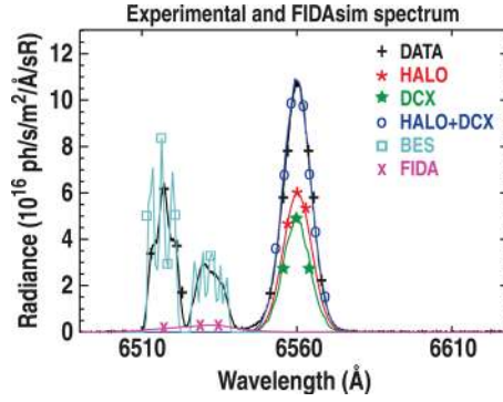
FIG. 5. Comparison of active spectral data with forward modeling with the FIDASim. The sum of halo and DCX intensity is in good agreement with the experimentally measured thermal spectral radiance.
