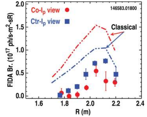
FIG. 16. Radial profile of fast-ion emission intensity FIDA at 1800 ms corresponding to Fig. 14(a). Measured FIDA emission is significantly below classical expectations indicative of fast-ion transport.
