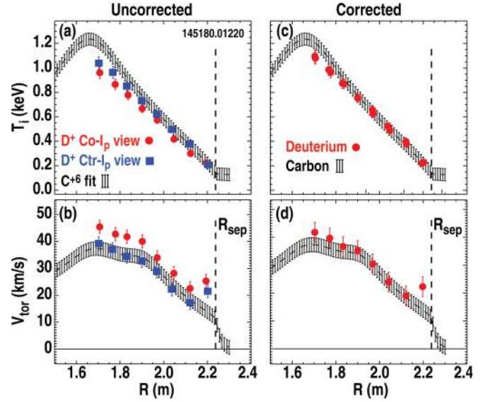
FIG. 6. Determination of deuterium temperature and toroidal rotation by correcting apparent values. (a) and (b) Profiles of apparent temperature and velocity from both co- I_p and ctr- I_p viewing D_\alpha systems, and spline fit of carbon temperature and carbon corrected velocity. (c) and (d) Profiles of corrected temperature and toroidal velocity, and carbon profiles [same as (a) and (b)].
