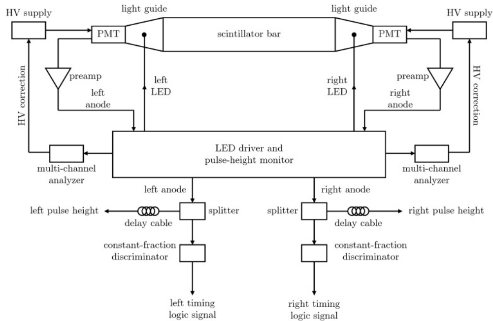
FIG. 7. Schematic diagram of the configuration of the electronics in the shielding hut for the front and rear array detectors. Note that the anode signals from the rear array detectors were not preamplified.
