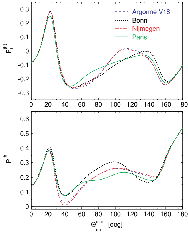
FIG. 33. (Color online) Comparison of FSI+MEC+IC+RC calculations of P_t^{(h)} (top panel) and P_l^{(h)} (bottom panel) for the Argonne V18, Bonn, Nijmegen, and Paris potentials. The results shown are for the central kinematics of our Q^2 = 1.136 (GeV/c) ^2 point and \phi_{np}^{c.m.} = 0^\circ .
