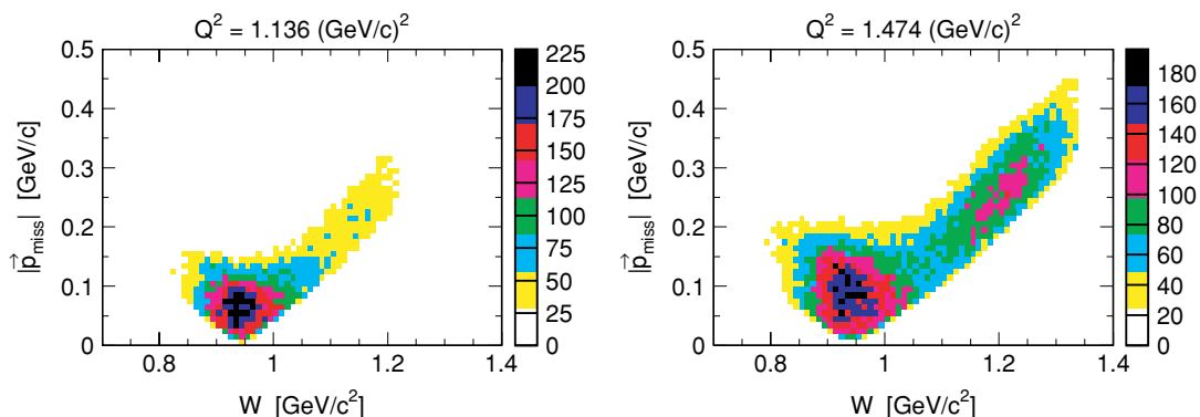
FIG. 12. (Color online) Correlation plot of |\mathbf{p}_{miss}| versus W for the full NPOL acceptance at Q^2 = 1.136 and 1.474 ( \text{GeV}/c^2 ) 2 .
