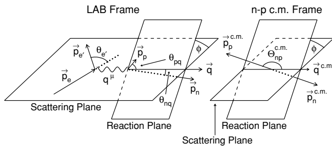
FIG. 30. Schematic diagram of the kinematics for the electrodisintegration of the deuteron in the one-photon exchange approximation as viewed from the laboratory frame and the recoiling n - p c.m. frame.
