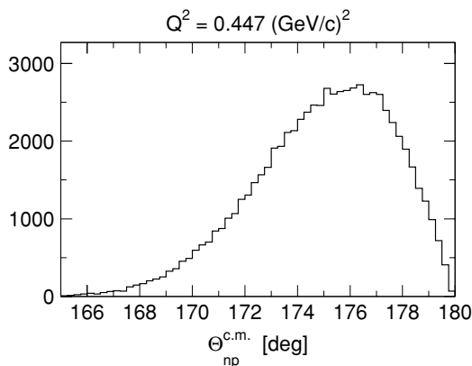
FIG. 23. Distributions of \Theta_{np}^{c.m.} after application of the final set of analysis cuts at Q^2 = 0.447 (\text{GeV}/c)^2 .
