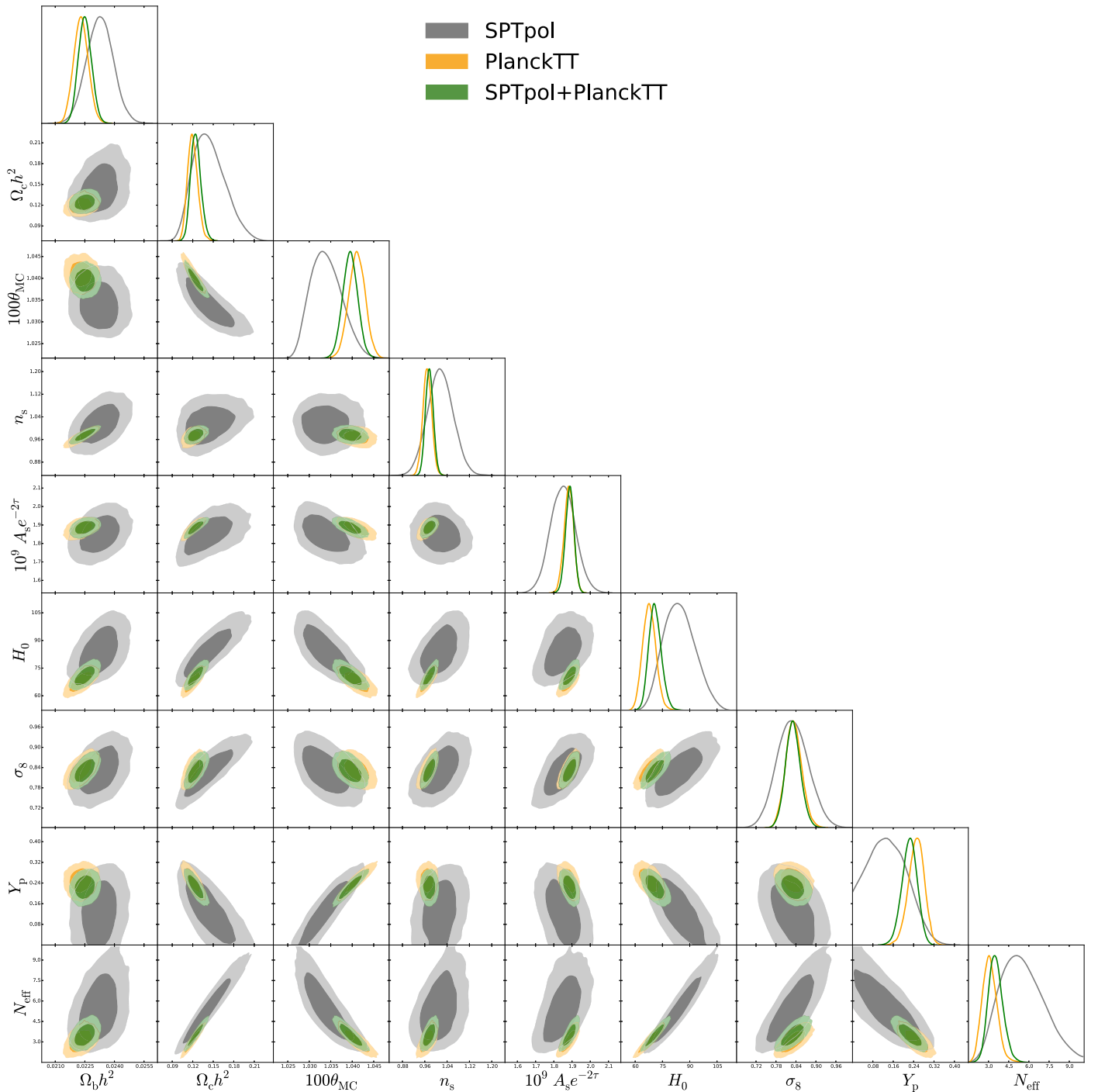
Figure 16. Marginalized parameter constraints for the \Lambda\text{CDM}+Y_p+N_{\text{eff}} model using SPTPOL, both independently and combined with PLANCKTT.
