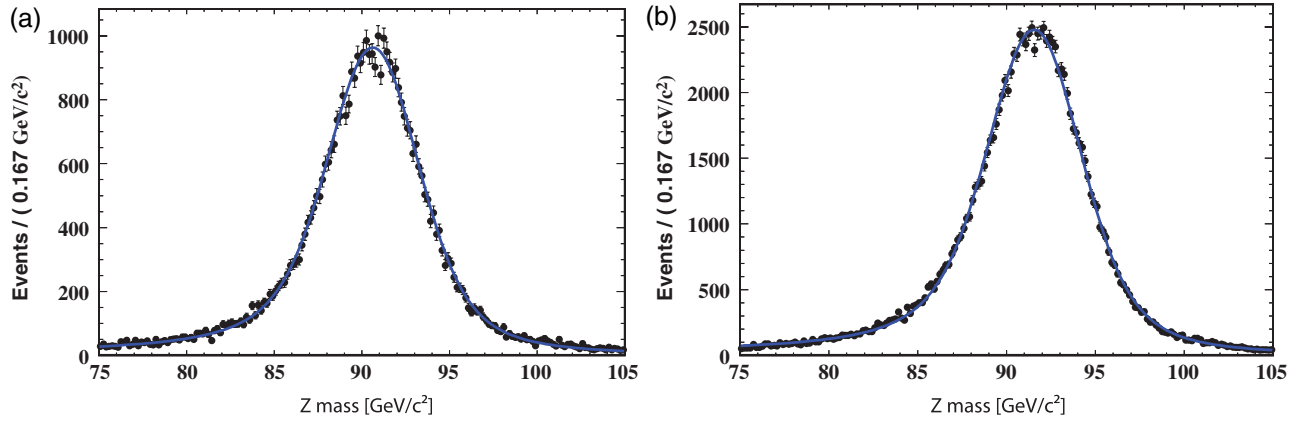
FIG. 11 (color online). (a): fit to the dilepton mass peak for electrons in data. (b): fit to the Z mass peak for electrons in simulation.
