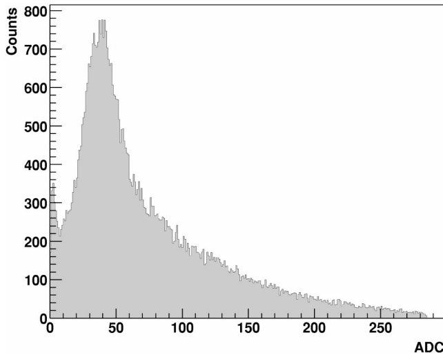
FIG. 1. Typical MIP spectrum. x-axis corresponds to ADC channel number. The hits correspond to isolated tracks with p > 1.25 GeV/ c which project to EMC towers. The peak corresponds to the energy deposited by nonshowering hadrons (MIP peak).
