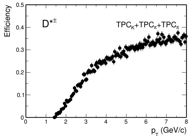
FIG. 10: Total D^* reconstruction efficiency versus D^* p_T .
