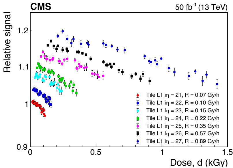
Figure 10. Relative signal for laser light versus accumulated dose for the SCSN-81 tiles in layer 1 with i\eta = 21-27 . The average dose rates are shown for each set of points. The vertical scale is logarithmic and subsequent sets are shifted up by a factor of 1.03 relative to the previous set for better visibility. Each set starts at the dose corresponding to integrated luminosity of 7 \text{ fb}^{-1} . Scaled statistical uncertainties are shown (see text).
