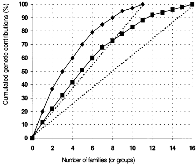
Figure 2. Cumulated genetic contributions of the families or the reproduction groups in two sheep breeds. Total number of groups is 11 for Solognote (◆) and 16 for Mérinos précoce (■).
