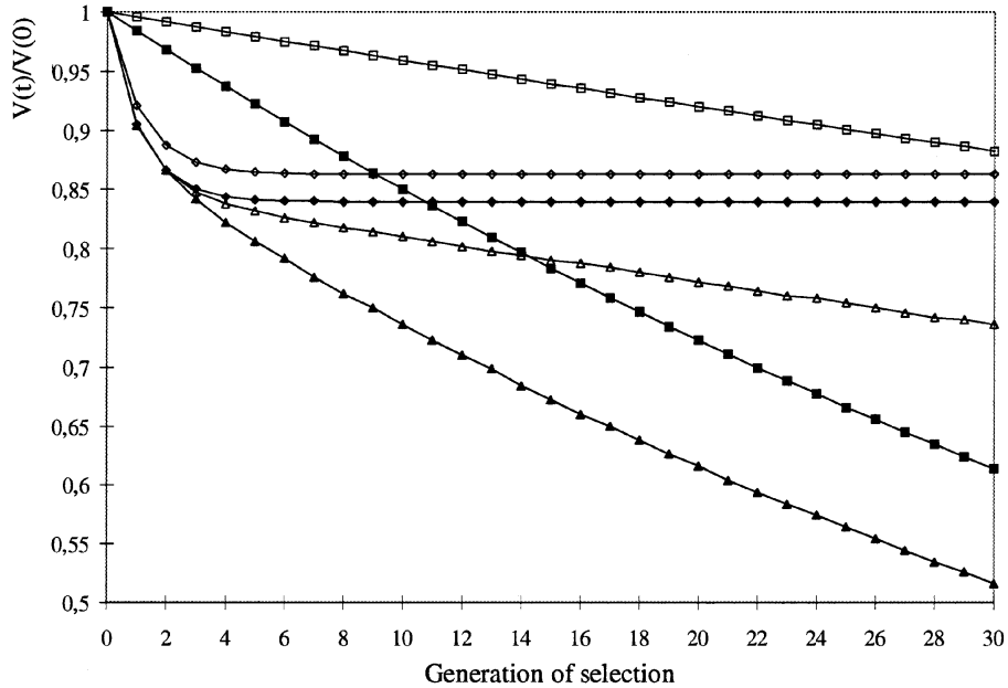
Figure 1. Evolution of genetic variance in three models, depending on effective population size N_e , with a proportion of selected males p (the proportion of females being 50%), for a trait with heritability 0.25 – W for Wright [53], with N_e = 120 ( \square ) or N_e = 31 ( \blacksquare ), B for Bulmer [3], with p = 50\% ( \diamond ) or p = 6.25\% ( \blacklozenge ), and V for Verrier et al. [49], with N_e = 120 and p = 6.25\% ( \triangle ) or N_e = 31 and p = 6.25\% ( \blacktriangle ).
