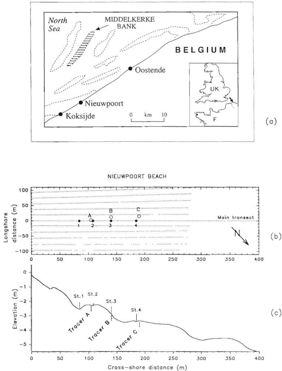
Figure 1. (a) Location map of the study area. Plan-view (b), and cross-sectional profile (c) of the intertidal zone of the experimental site. Locations of instrument stations (St. 1, 2, 3 and 4) and sand tracer injection points (tracer A, B and C) are shown on (b) and (c), respectively. Dashed lines on (b) indicate locations of topographic survey transects.
