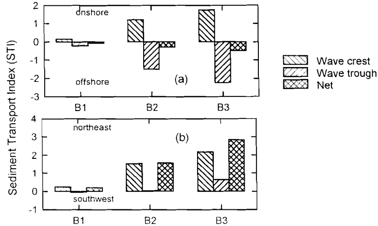
Figure 8. Top: Sand Transport Indices (STI) beneath a wave crest (open circles) and a wave trough (solid circles) in the alongshore (a) and cross-shore (b) directions respectively. Bottom: Average value of STI for the tracer B experiment period, along the cross-shore (a) and longshore (b) directions for wave crests, troughs and their vector sum (net), respectively.
