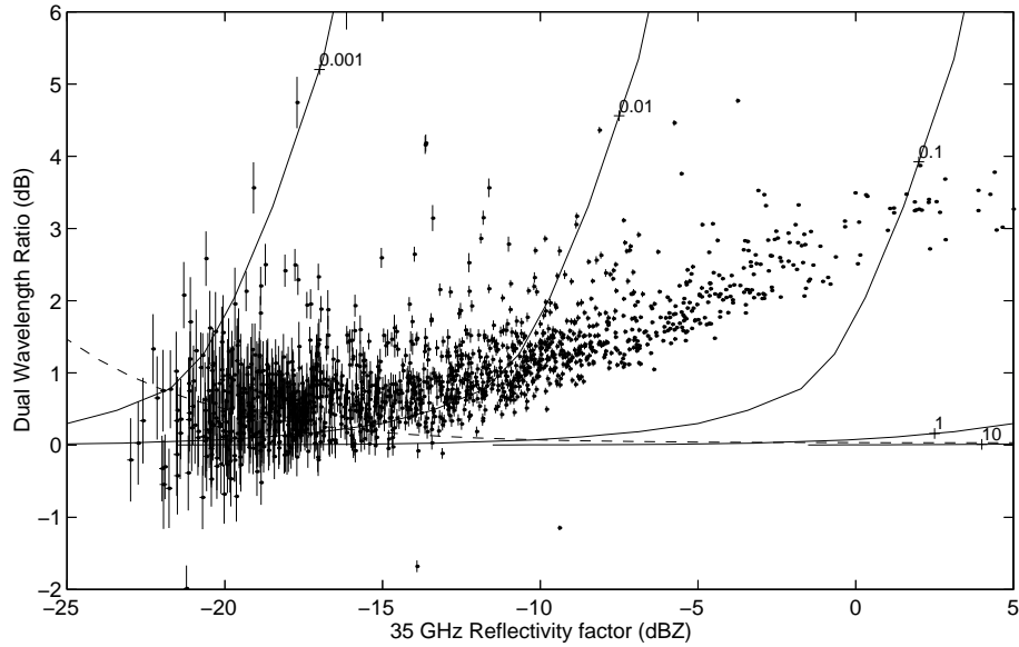
FIG. 6: Scatterplot of Z_{35} versus DWR for the data presented in Fig. 5 with lines of constant IWC (labelled in \text{g m}^{-3} ) overlaid. The error bars have been calculated assuming all pulses are independent, and the dashed line indicates the threshold for the rejection of data for the purposes of size retrieval, at an altitude of 7 km.
