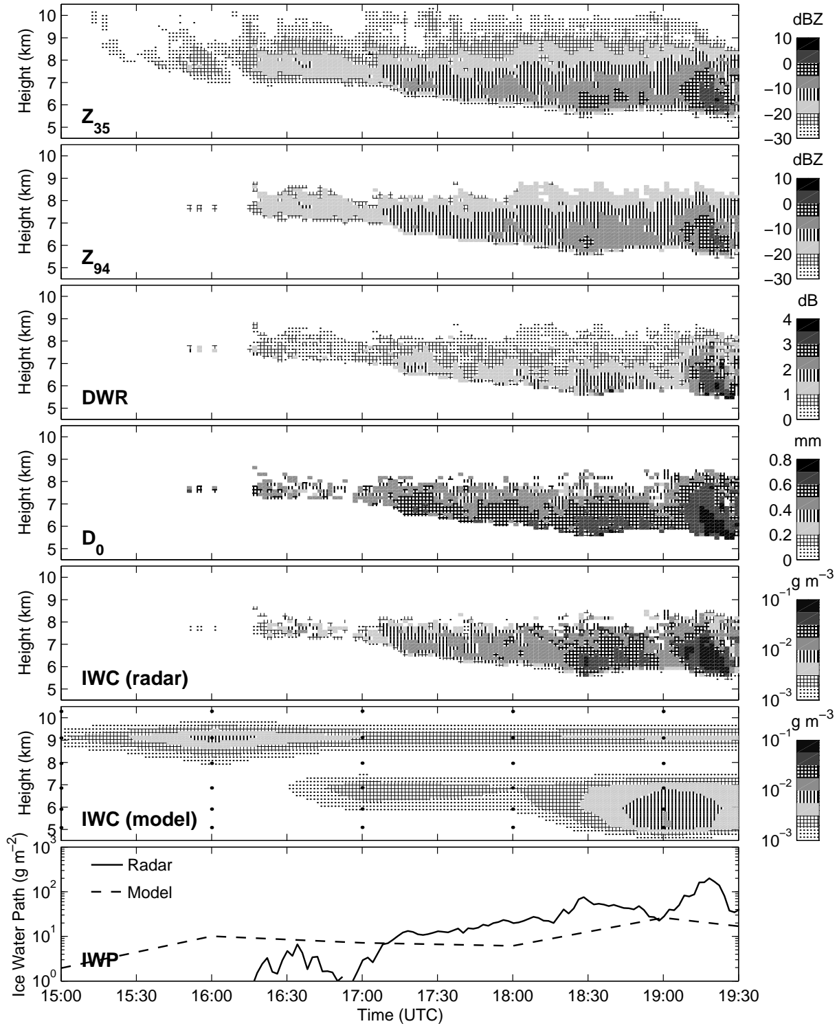
FIG. 5: Time-series of dual-wavelength radar data and derived quantities obtained on 22 June 1996: (from top) 35 GHz reflectivity factor; 94 GHz reflectivity factor; dual-wavelength ratio; median volume diameter; ice water content derived from radar; ice water content diagnosed by the UKMO Unified Model (where the black dots indicate the model gridpoints); ice water path from the model and the radar.
