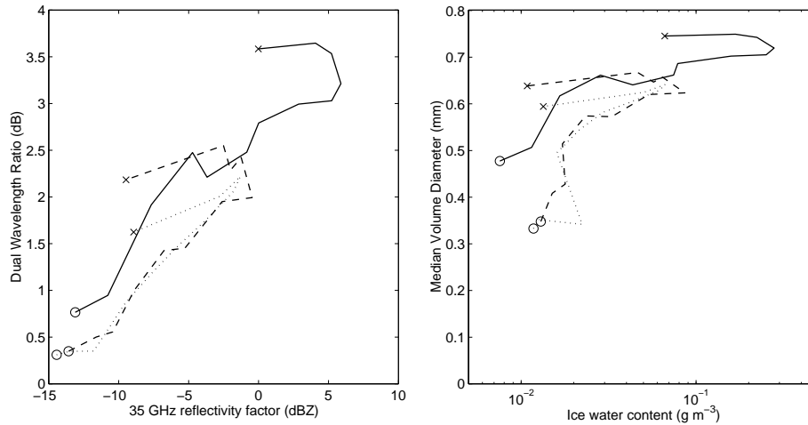
FIG. 8: DWR against Z_{35} , and D_0 against IWC for the three fallstreaks highlighted in Fig. 7, using the same line-styles. The circles indicate the top of the streaks and the crosses indicate the bottom.
