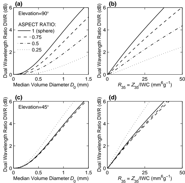
FIG. 2: DWR as a function of D_0 and R_{35} at vertical incidence (top row) and at an elevation of 45° (bottom row), for oblate crystals of four different aspect ratios. The radiation is vertically polarized at both wavelengths and the distribution is exponential.
