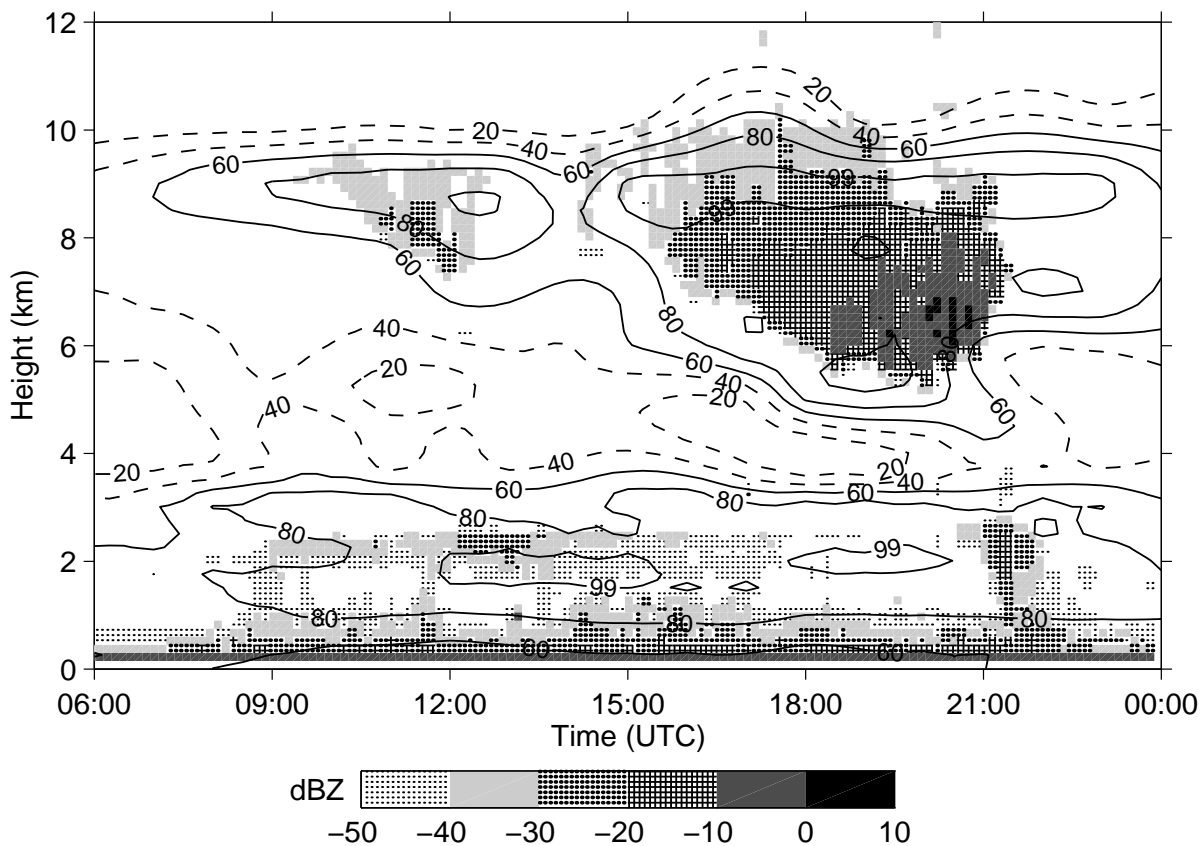
FIG. 4: 35 GHz reflectivity factor with UKMO Unified Model relative humidity contours (%) superimposed, for part of 22 June 1996.
