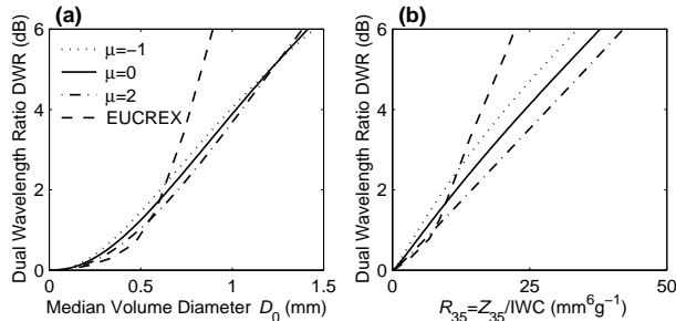
FIG. 3: DWR as a function of D_0 and R_{35} for gamma distributions with three values of the shape parameter \mu , and as derived empirically from real size spectra measured during EUCREX.
