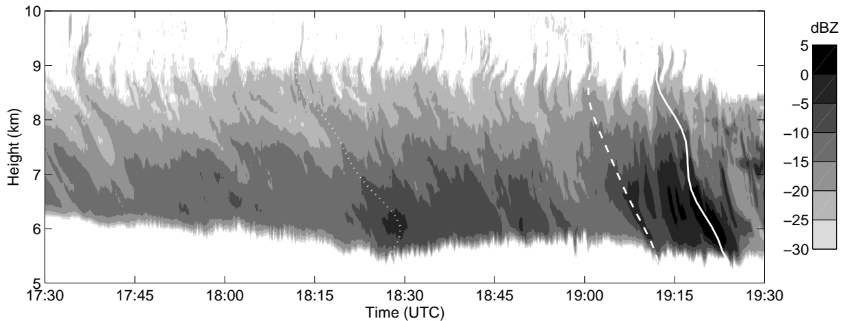
FIG. 7: High resolution 35 GHz reflectivity factor with objectively-derived fallstreaks overlaid.
