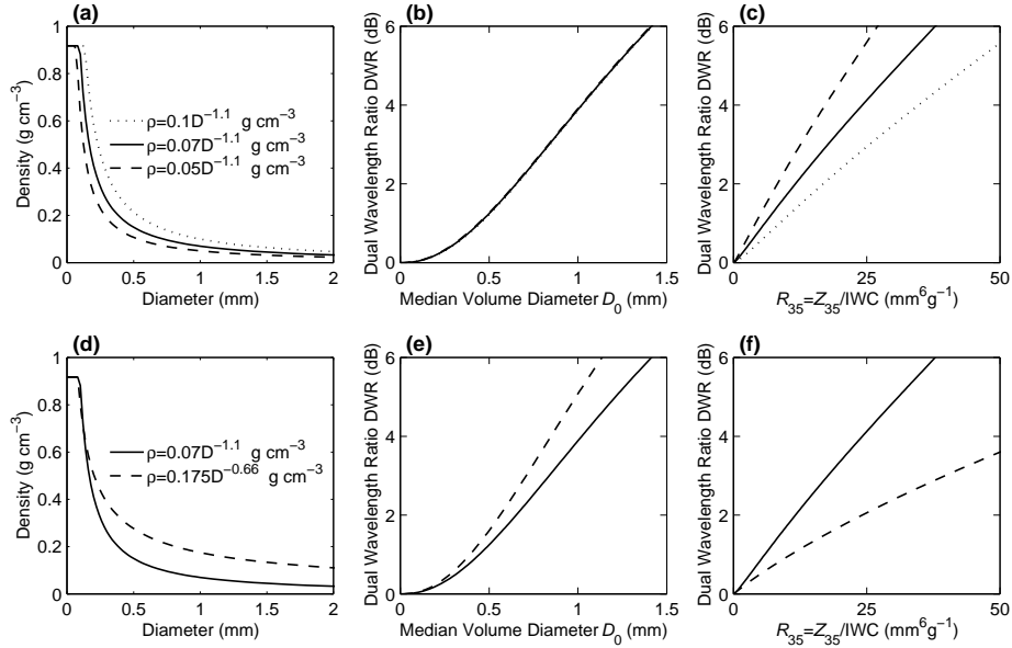
FIG. 1: The sensitivity of dual-wavelength retrieved quantities to density, for an exponential distribution of ice crystals. The density functions described in the text are plotted in (a) and (d), with DWR as a function of D_0 and R_{35} to their right.
