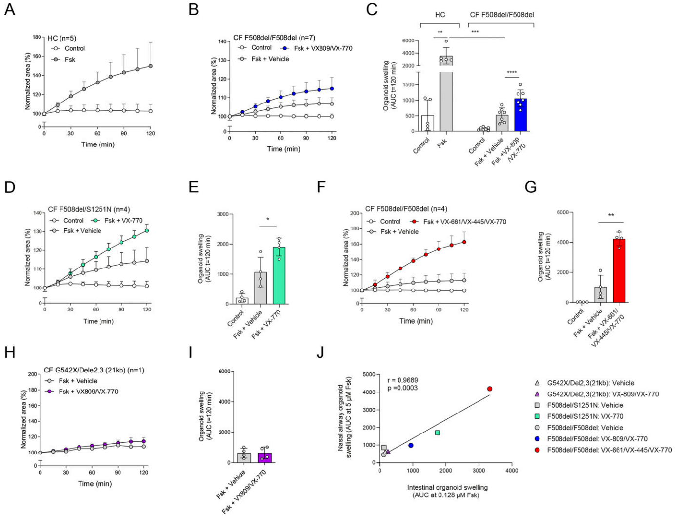
Figure 3. Validation of CFTR modulator responses in NR/IL-1 \beta -cultured nasal-airway organoids (NAOs).
