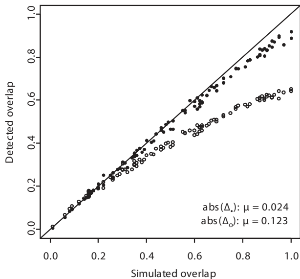
Figure 2 Agreement between simulated and detected niche overlap. Each dot corresponds to a pair of simulated entities. Simulated overlap corresponds to the volume in common between the two bivariate normal distributions with different means on precipitation and temperature gradients (see Figure 1). Filled circles represent the detected overlap with correction for climate availability (density of occurrences divided by the density of climate across the entire climate space). Open circles show the detected overlap when no correction for climate availability is applied. The average absolute difference between the simulated and measured overlap ( \text{abs}(\Delta); \mu ) is indicated for both corrected and uncorrected measures.
