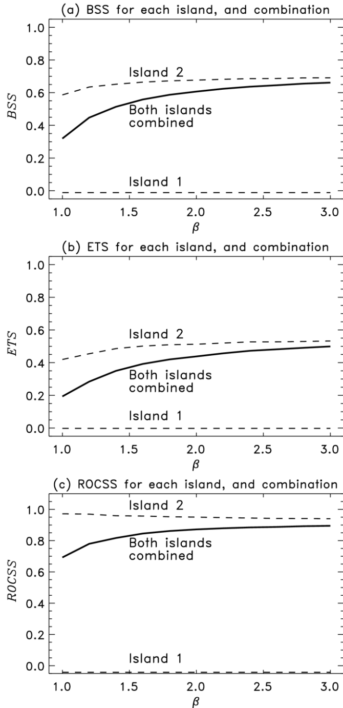
Figure 3. Scores for three verification metrics when applied separately to forecasts at islands 1 and 2, and when combined using the conventional methods of calculation: (a) Brier skill score (BSS); (b) equitable threat score (ETS) and (c) the ROC Skill Score (ROCSS). Scores are shown for a range of standard deviations \beta at island 2. See Figure 2 and subsection 3(b) for more on the experimental design.
