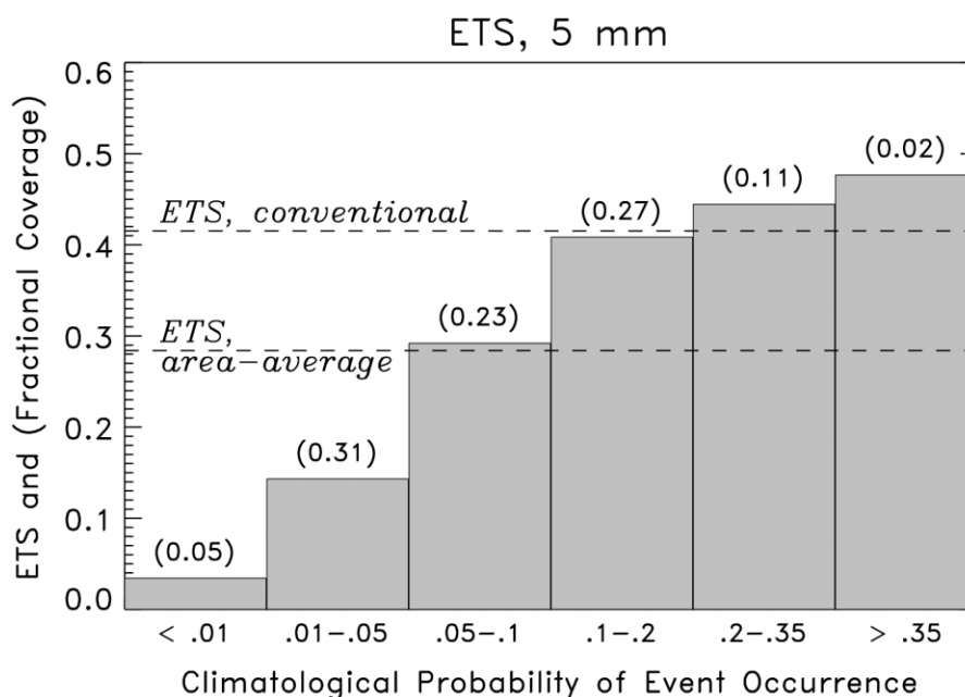
Figure 5. Equitable threat scores (ETSs) of forecasts of precipitation exceeding 5 mm when divided into six categories based on the climatological probability of the event occurring. Forecasted and analysed data are from January and February 1979–2003 over the conterminous USA. Brackets contain the proportion of grid points occurring in each category. The upper dashed line shows the ETS calculated using the conventional method (Eq. (17)) and the lower dashed line the area-averaged (population-weighted) ETS (Eq. (19)).
