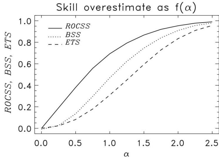
Figure 1. Three conventional verification metrics as functions of the parameter \alpha : relative operating characteristic skill score (ROCSS), Brier skill score (BSS) and equitable threat score (ETS). The parameter \alpha describes the mean observed climatological value (say of temperature) at island 1, while island 2 has a mean value of -\alpha .
