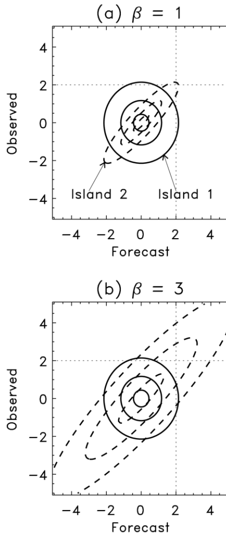
Figure 2. Illustration of experimental design (see subsection 3(b) of the text). Forecasts of temperature are simulated at two hypothetical islands. The first island has forecasts and observations which are uncorrelated; the second island has forecasts and observations correlated at 0.90. On both islands, the observed and forecasted values are both normally distributed about the mean, which is taken as zero. The standard deviation \beta for forecasts and observations is fixed at 1.0 in panel (a) for both islands. In panel (b), \beta is fixed at 1.0 for island 1 and 3.0 for island 2. Dotted lines indicate the event threshold of the forecasted or observed temperature being greater than 2.0.
