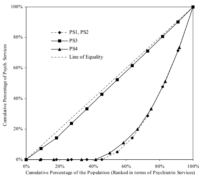
Figure 1 Lorenz Curves for illustrative data on four distributions of psychiatric services
