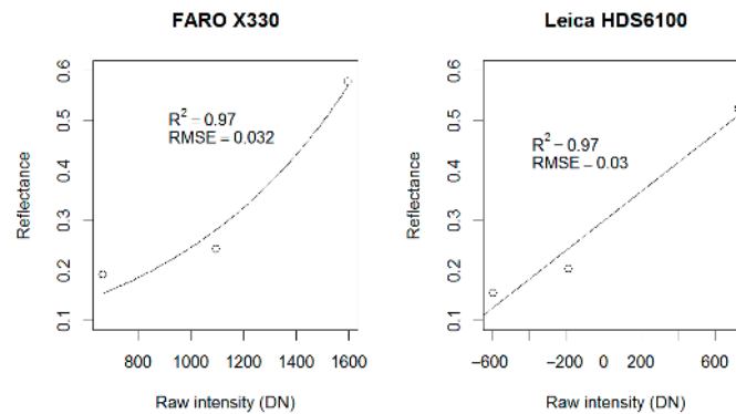
Figure 3. Raw intensity measurements presented against measured reflectance of the Spectralon reflectance panels (50%, 25%, 12%) with the regression models, and respective coefficient of determinations ( R^2 ) and root mean square errors (RMSE), between raw intensity (digital number, DN) and reflectance for the FARO and Leica scanners, respectively.
