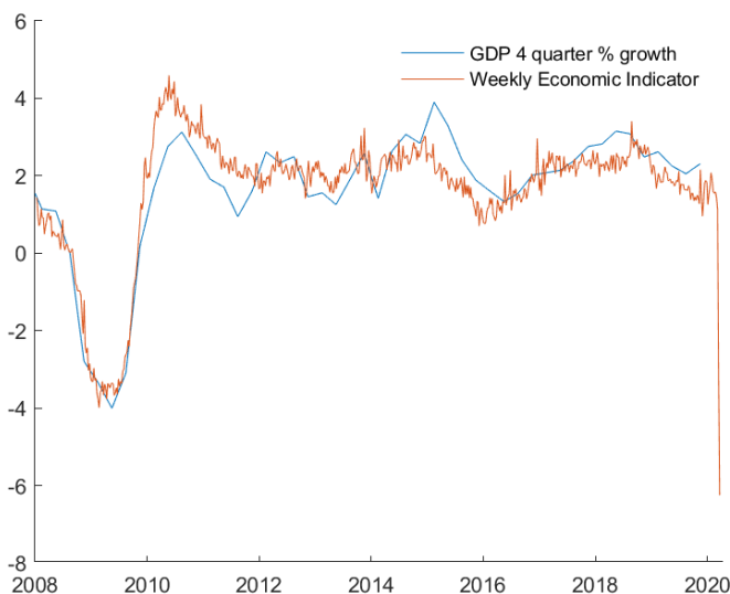
Figure 4: WEI and GDP growth
