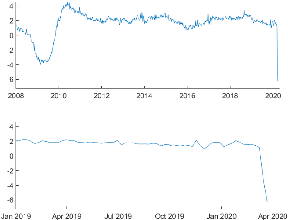
Figure 1: Weekly Economic Indicator (WEI)
