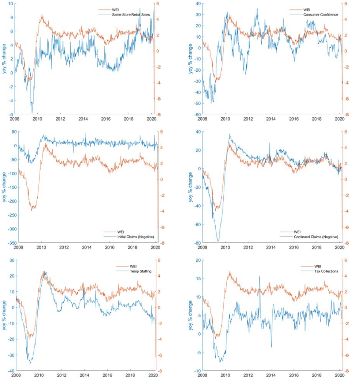
Figure 2 Weekly Variables and WEI
