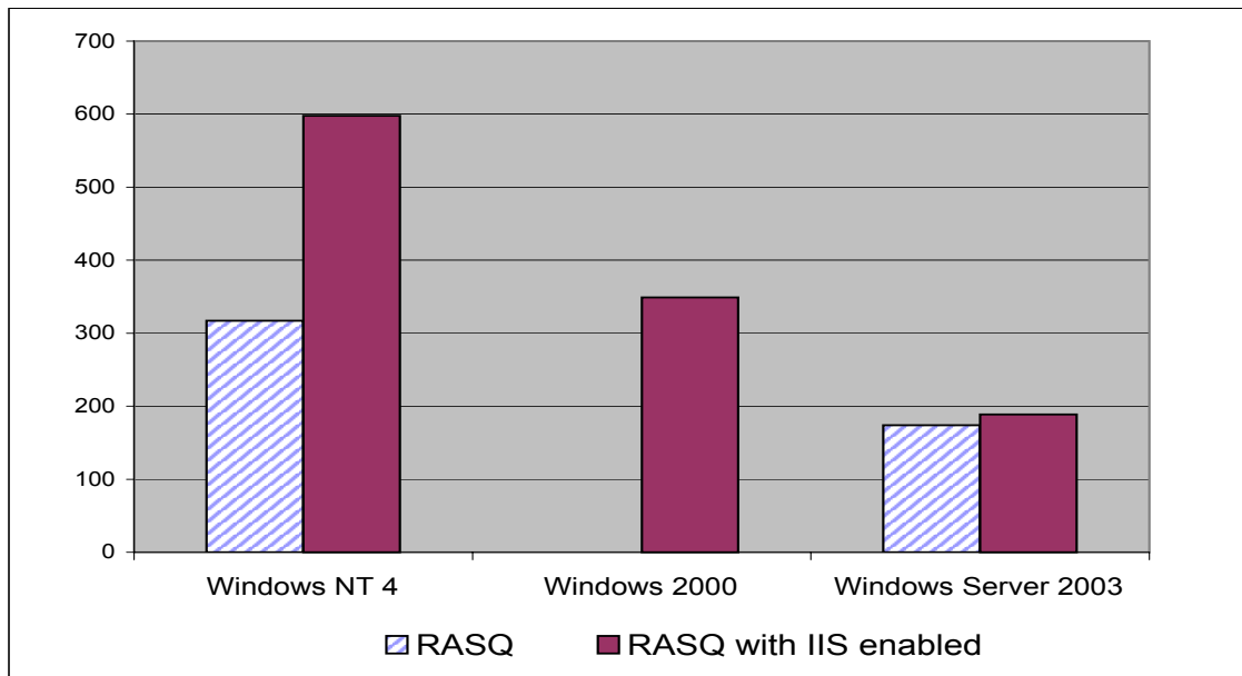
Fig. 1. Relative Attack Surface Quotient of Different Versions of Windows
