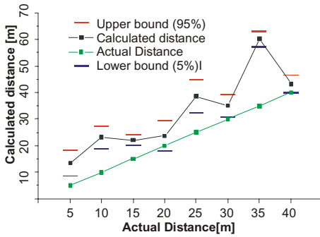
Fig. 4. Distance as calculated from RTT versus actual distance between both nodes. 95% confidence levels are given Fig. 5. Received signal strength indicator versus distance. Confidence intervals are too small to be shown
