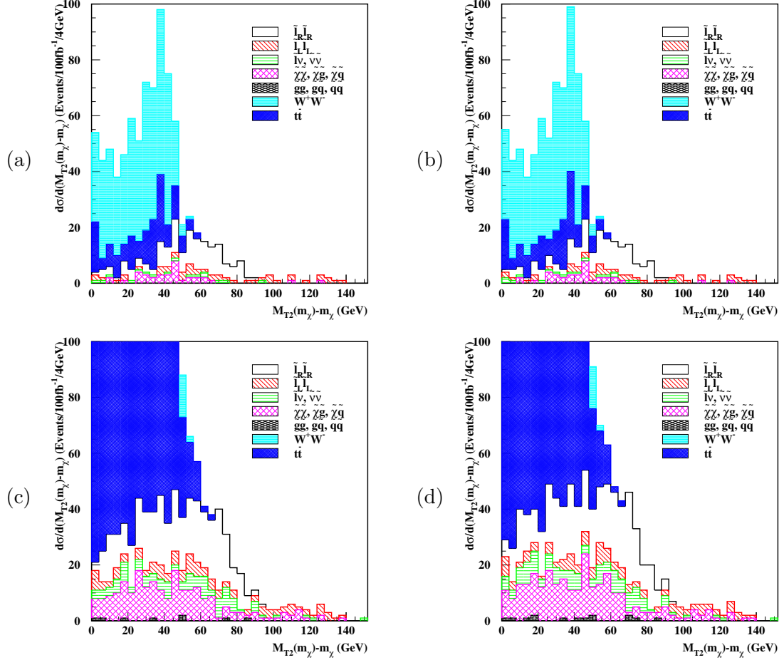
Figure 8: These M_{T2} distributions for O1 are generated from 100 \text{ fb}^{-1} at high luminosity, and from the M_{T2} cuts described in section 3.4. (a) and (b) use the “hard” cuts, while (c) and (d) use the “soft” cuts. In (a) and (c), events containing a jet with p_T > 40 \text{ GeV} were vetoed. In (b) and (d), this cut was relaxed to 50 \text{ GeV} . In all plots, M_{T2}(\chi) is evaluated at \chi = m_{\tilde{\chi}_1^0} . The results are presented in the form M_{T2}(m_{\tilde{\chi}_1^0}) - m_{\tilde{\chi}_1^0} in order to show the edge of the signal region located at the difference between the slepton and neutralino masses ( 92.5 \text{ GeV} ).
