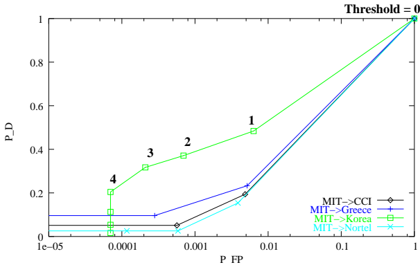
Figure 16: Receiver operating characteristics using a 30-minute advertisement window of failure observation. For paths where many failures happen in a short time span, failures can be a good predictor of future failures.
