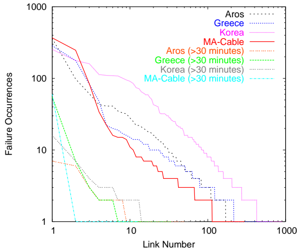
Figure 6: Failures appear in many different places, regardless of failure duration.
