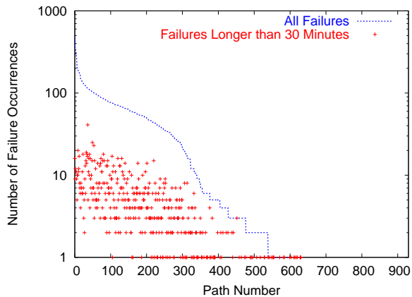
Figure 9: The success of a reactive routing network depends on which paths commonly experience failures. This figure ranks the 930 paths according to the number of failures that each path experiences, for various failure durations (approximately 300 paths did not experience failures during the collection period).
