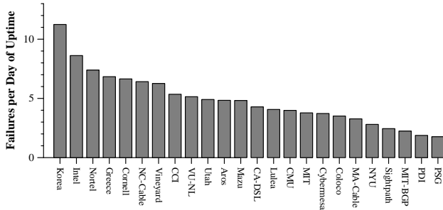
Figure 5: Failures per day of uptime by measurement host. (Seven recently added sites have very few failures to date, and thus are not shown.)
