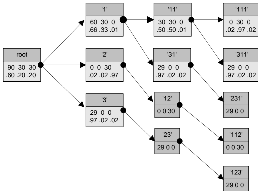
Figure A.1: A VOM model (tree) generated from 30 consecutive repetitions of the pattern “11123”. The first line of numbers below the node's (shaded) label present the three counts ordered with respect to symbols {1,2,3} conditioned on the context that is represented by the label. The second line of numbers below the node label presents the three predictors. Truncated nodes are shaded.
