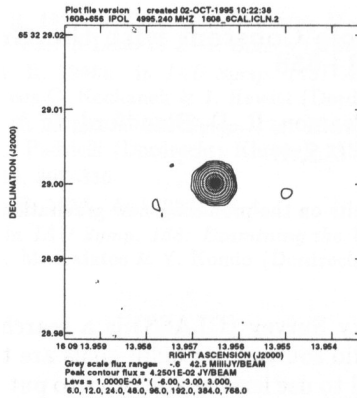
Figure 1. 5 GHz VLBA image of component A in 1608+656. The rms noise in the map is \sim 0.1 mJy, giving a dynamic range >400:1 . The component is well fitted by a point source; no extended emission is seen. The images of the other components have similar characteristics.
