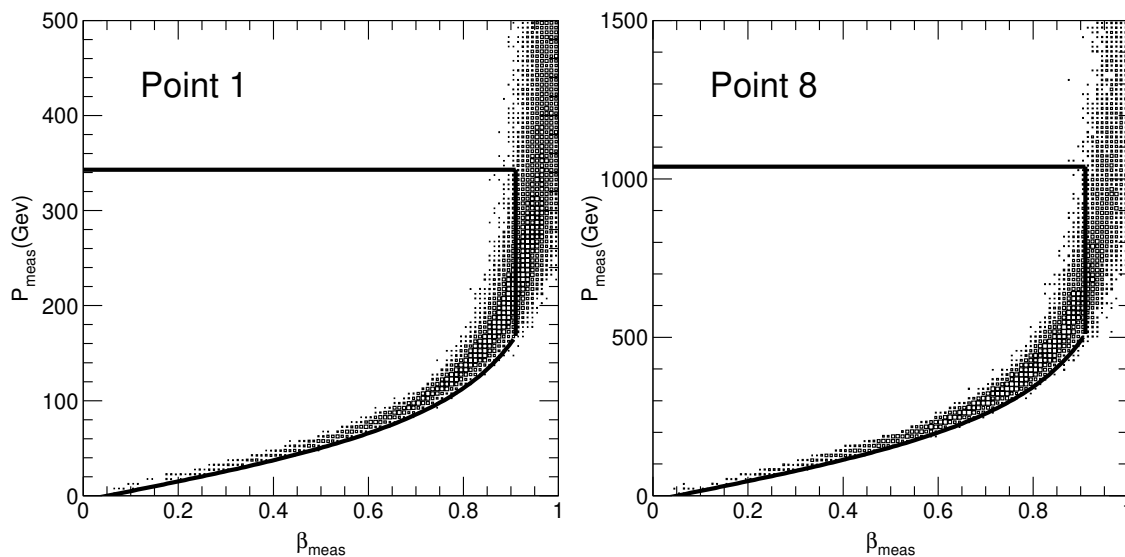
Figure 3: Distribution of P_{\text{meas}} versus measured \beta_{\text{meas}} for sleptons, for Points 1 and 8. The region to the left of the thick lines in the (\beta_{\text{meas}}, P_{\text{meas}}) plane defines the selected slepton candidates.
