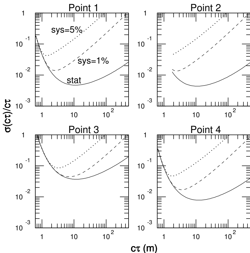
Figure 6: Fractional error on the measurement of the slepton lifetime c\tau , for model points 1 to 4. We assume an integrated luminosity of 30 \text{ fb}^{-1} . The curves are shown for three different assumptions on the fractional systematic error on the R measurement: statistical error only (full line), 1% systematic error (dashed line), 5% systematic error (dotted line).
