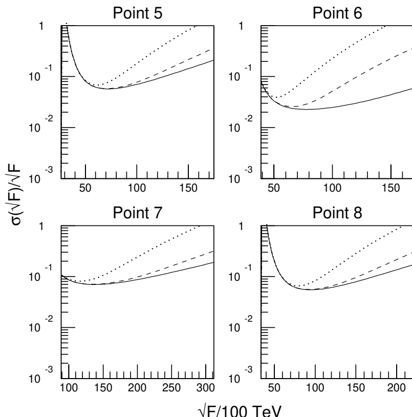
Figure 12: The same as in figure 11, but for model points 5 to 8.
