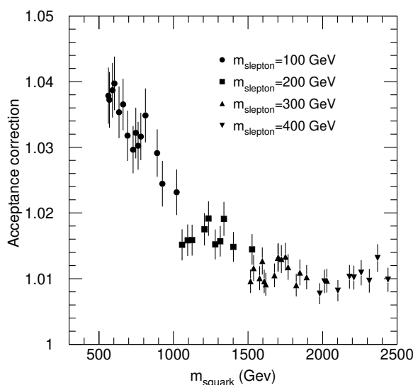
Figure 10: Acceptance correction factor calculated for 50 different GMSB models. The effects of the loss of low momentum sleptons and of the \eta acceptance are included. The acceptance is given as a function of the squark mass.
