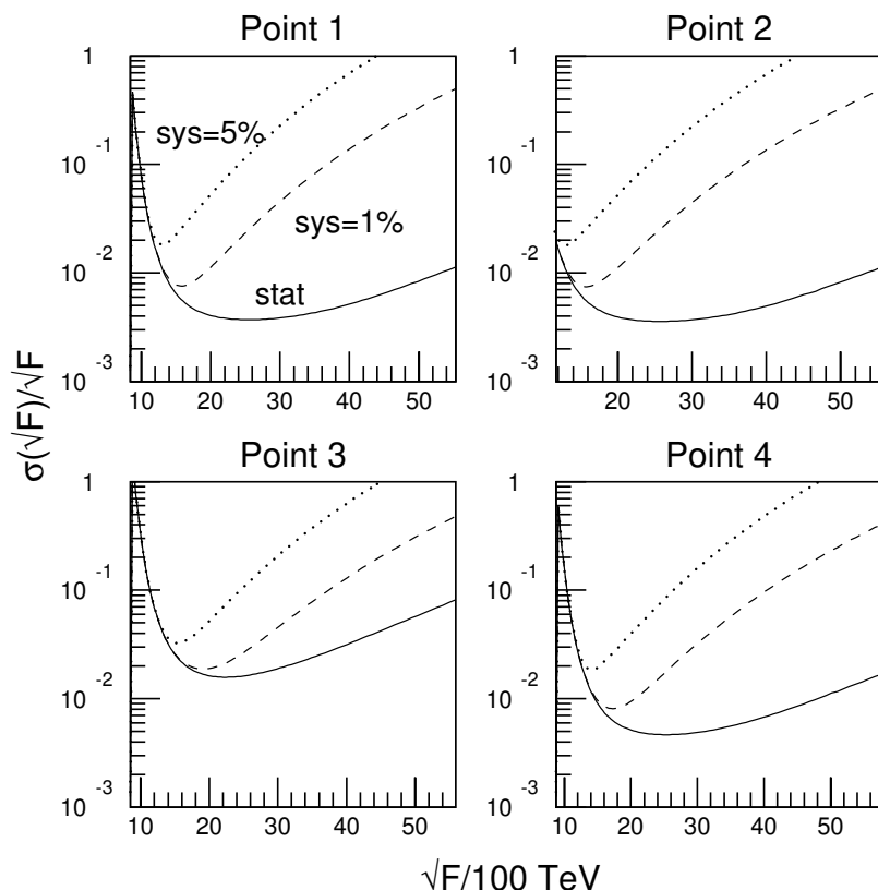
Figure 11: Fractional error on the measurement of the SUSY breaking scale \sqrt{F} for model points 1 to 4. We assume an integrated luminosity of 30 \text{ fb}^{-1} . The curves are shown for the three different assumptions on the fractional systematic error used in figures 6 and 7.
