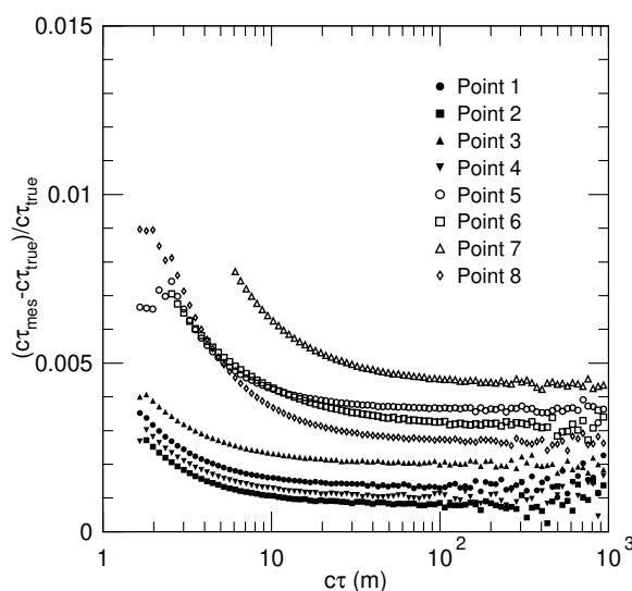
Figure 9: Fractional deviation of the c\tau value measured using the momentum distribution of the candidates from the true value as a function of c\tau . The different curves shown are for the 8 example points considered. The statistical error and the systematic uncertainty on N_2 are not included in the calculation.
