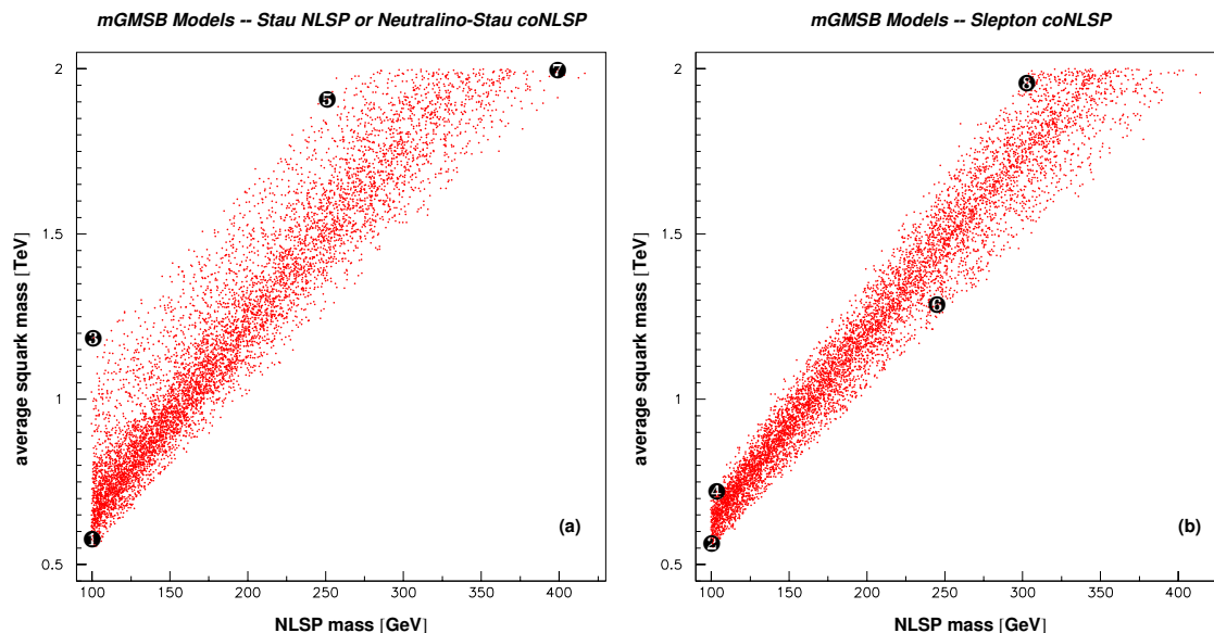
Figure 1: Scatter plots in the (m_{\text{NLSP}}, m_{\bar{q}}) plane for all relevant GMSB models generated. a) stau NLSP or neutralino-stau NLSP scenarios; b) slepton co-NLSP scenario. The eight sample models of tables 1 and 2 are highlighted with their reference number.
