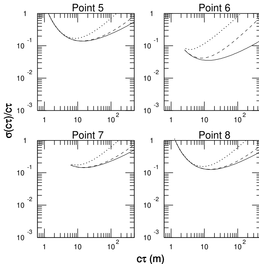
Figure 7: The same as in figure 6, but for model points 5 to 8.
