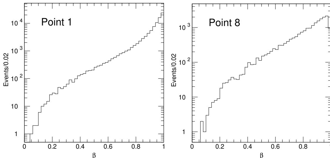
Figure 2: Distribution of \beta for the NLSP sleptons at Points 1 and 8.
