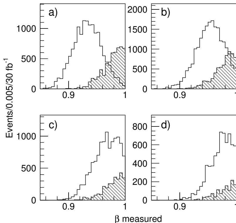
Figure 8: \beta distributions for sleptons (full line histogram) and background muons (hatched histogram) for model point 4. The distributions are given for four momentum bins: a) 250 < p < 300 GeV, 300 < p < 400 GeV, 400 < p < 500 GeV, 500 < p < 600 GeV. The histogram limits exclude the peak at \beta = 1 for the background.
