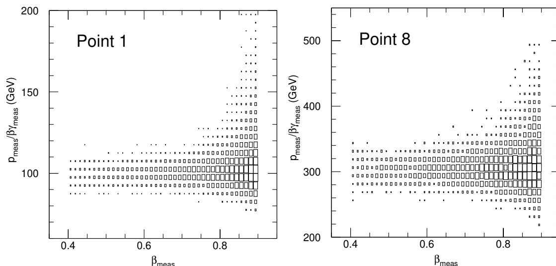
Figure 4: Distribution of the measured mass values for Points 1 and 8 as a function of \beta . The number of events in the scatter plot is arbitrary.
