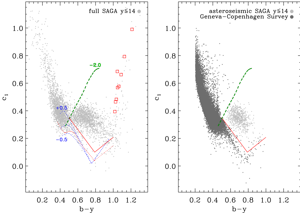
Figure 5. Left-hand panel: b - y versus c_1 plane for the entire SAGA photometric catalogue with y \leq 14 and Pflag=0 . Dotted red line is the main-sequence fiducial of Olsen (1984), while the continuous red line is the +0.06 mag shift we use to separate dwarfs from giants. Open squares are cool M giants, also from Olsen (1984). For reference, the metallicity-dependent dwarf sequences of Árnadóttir et al. (2010) are also shown (in blue, for -0.5 \leq [Fe/H] \leq 0.5 as indicated), as well as the metal-poor ( [Fe/H] = -2.0 ) red giant branch sequence of Anthony-Twarog & Twarog (1994). Right-hand panel: dark-grey circles identify all dwarf/subgiant stars in the Geneva-Copenhagen Survey, most of the late-type ones being successfully delimited by our shifted fiducial (in red). Pale-grey circles are all asteroseismic giants having good photometric and metallicity flags and y \leq 14 .
