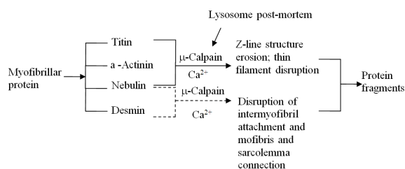
Fig. 3: Mechanism of calpain catalyzed meat proteolysis (Tarte and Amundson, 2006)
