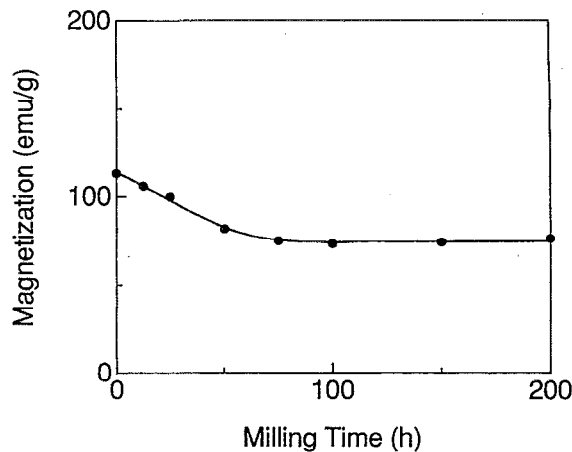
FIG. 2. Saturation magnetization as a function of milling time for the X=50 powders.
