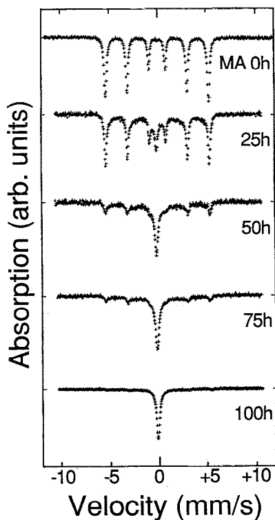
FIG. 6. ^{57}\text{Fe} Mössbauer spectra for the X=70 powders subjected to MA for different milling times.
