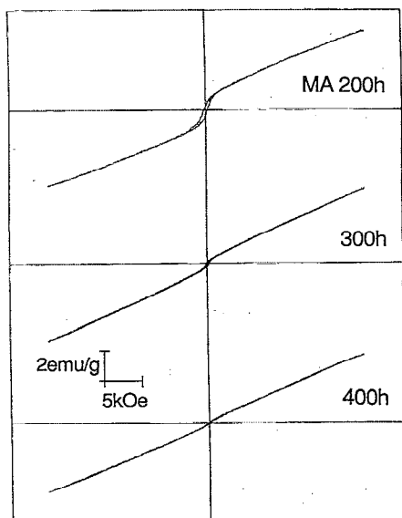
FIG. 7. Magnetization curves for the X=70 powders subjected to MA for different milling times.
