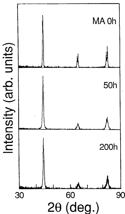
FIG. 1. X-ray diffraction spectra for the X=50 powders subjected to MA for different milling times.
