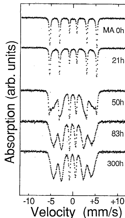
FIG. 5. ^{57}\text{Fe} Mössbauer spectra for the X=20 powders subjected to MA for different milling times.
