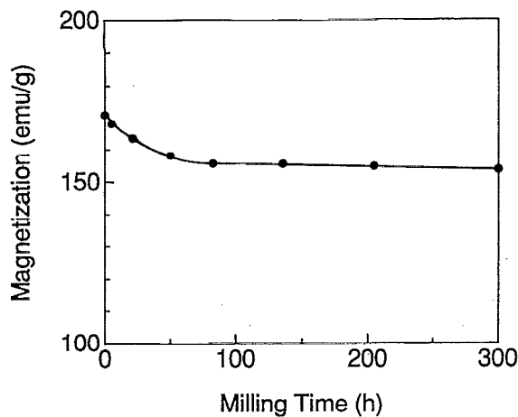
FIG. 4. Saturation magnetization as a function of milling time for the X=20 powders.
