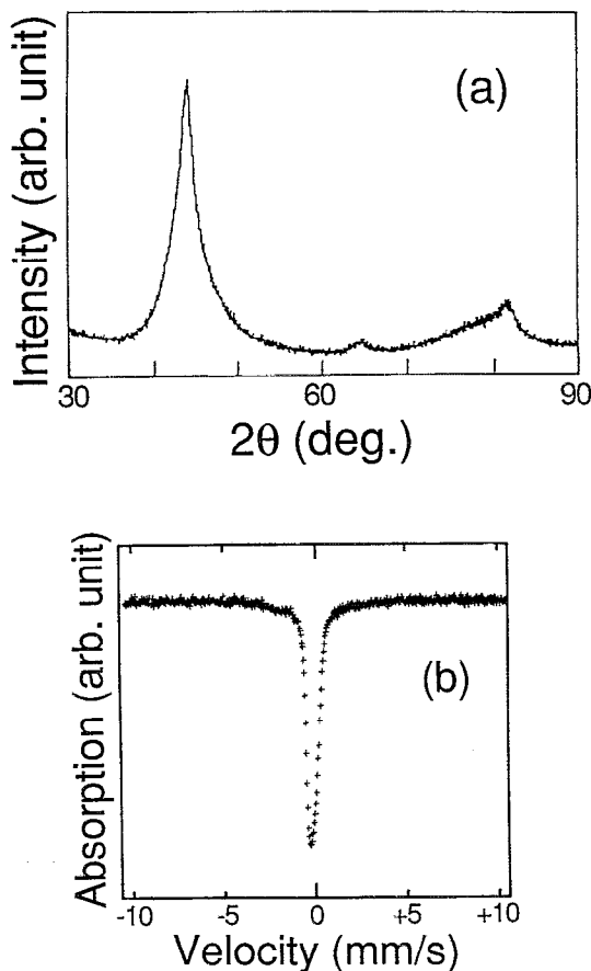
FIG. 8. (a) X-ray diffraction spectrum and (b) ^{57}\text{Fe} Mössbauer spectrum for the X=50 powders ball milled in Ar gas for 200 h and further milled in \text{N}_2 gas atmosphere. Nitrogen content is 5.8 at. %.
