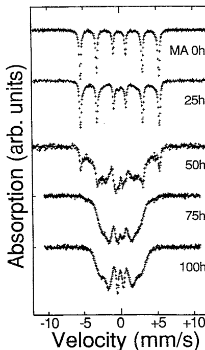
FIG. 3. ^{57}\text{Fe} Mössbauer spectra for the X=50 powders subjected to MA for different milling times.
