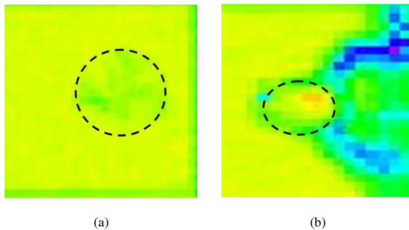
Fig. 18. Comparison of damaged area of spot-welded (a) and mechanically fastened (b) joints after DLS tests. The black dashed lines indicate the welded area (a) and deformed fastener hole (b) after DLS tests, respectively.
