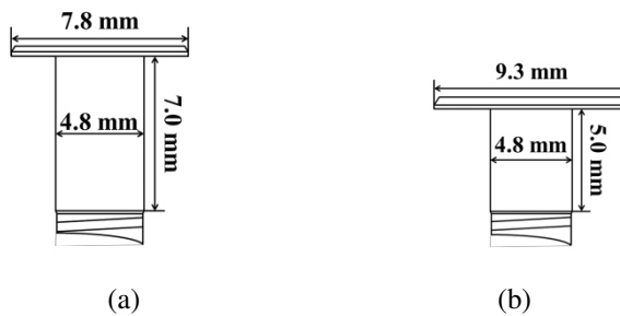
Fig. 6. Schematic of the Hi-Lok ® fasteners utilized in the mechanical tests: (a) HL10V6; (b) HL12V6.
