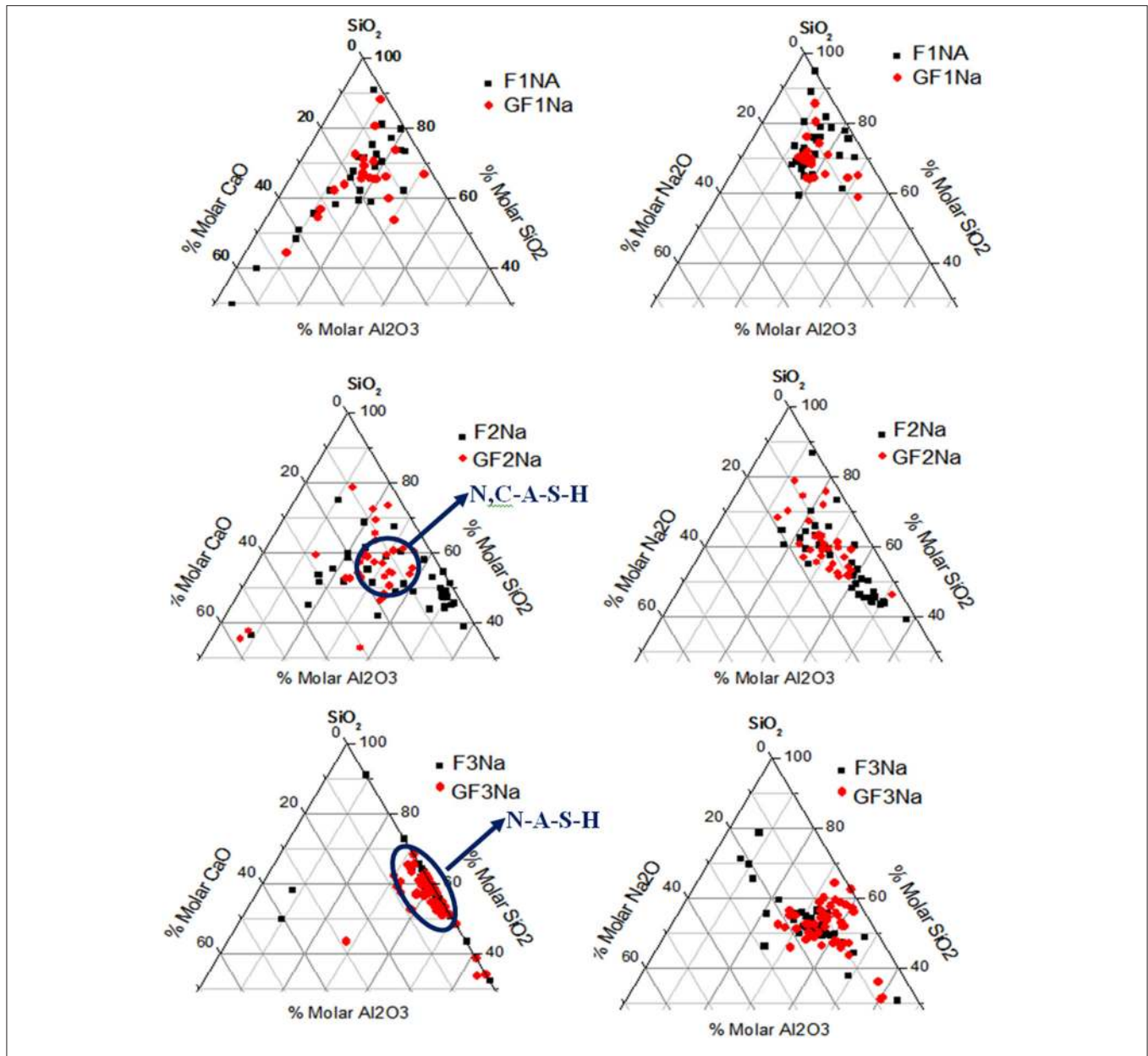
FIGURE 9 | EDX chemical composition of gels formed (qualitative data).
