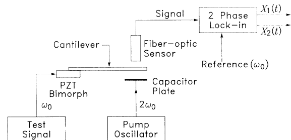
FIG. 1. Block diagram of the mechanical parametric amplifier and associated measurement apparatus. The spring constant of the cantilever is modified (pumped) at frequency 2\omega_0 by the electric field from the capacitor plate.
