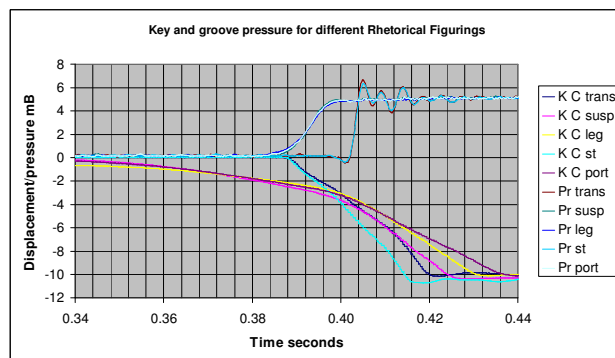
Fig 9 Graph showing key movements (K) and pressure in the groove (Pr) for the first note of a theme played with the Rhetorical Figures Transitus, Suspriatio, Legato, Staccato and Portato. Pressure curves aligned to highlight similarity. Örgryte Church, Göteborg
