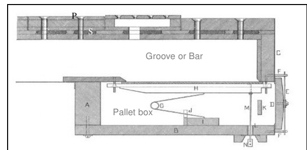
Fig 1 Cross section of a bar (groove) and slider windchest adapted from Audsley Fig CLIX. The significant parts are: N connected to the tracker from the key and pulling open pallet H via tracker M, compass spring G providing the closing force on the pallet, pallet box containing pressurised air, bar connecting all pipes played with one key, slider S shown open so that the pipe, planted in tapered hole P, will speak when the pallet is opened
