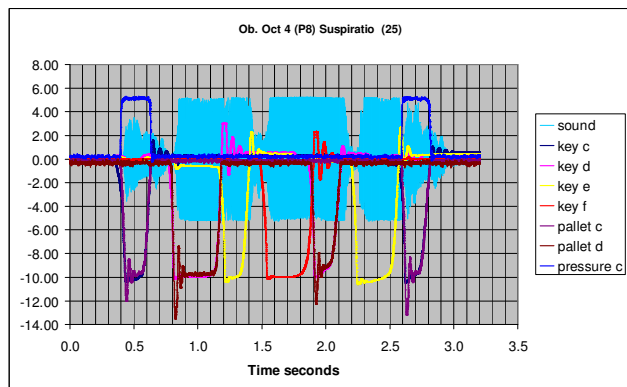
Fig 7 Graph showing the key and pallet movements, pressure in the groove and sound recording for a theme played with Suspriatio Rhetorical Figure. Örgryte Church, Göteborg
