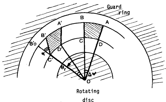
Fig. 7. Skin surface deformation during torque application \alpha : shear angle of an infinitesimal element (i.e., area ABCD which becomes A'B'C'D'). \theta(r) : rotation angle of skin at radius r
