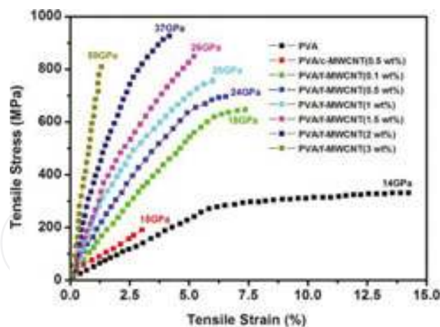
Figure 21. Stress-strain curves of PVA/f-MWCNTs composite fibers, the values on the tips of curves are Young's modulus of the corresponding fibers [29].
