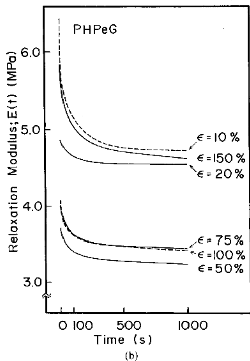
Figure 5. Change in relaxation modulus E(t) at various strains of (a) skin-type PHPeG-82 membrane and of (b) elastomer-type PHPeG membrane in PEFC solution at 25°C.
