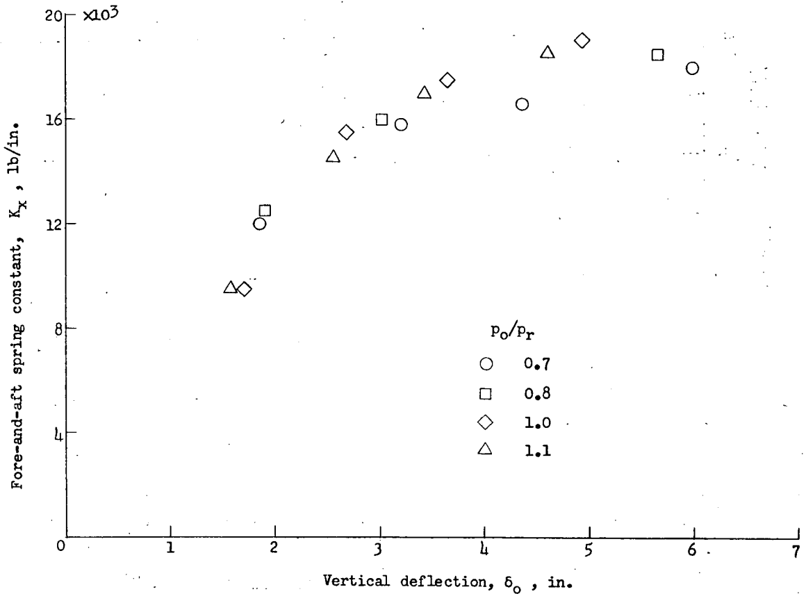
Figure 31.- Experimental variation of fore-and-aft spring constant with vertical deflection and inflation pressure for a 56x16-32PR-VII tire. (Data from ref. 21.)
