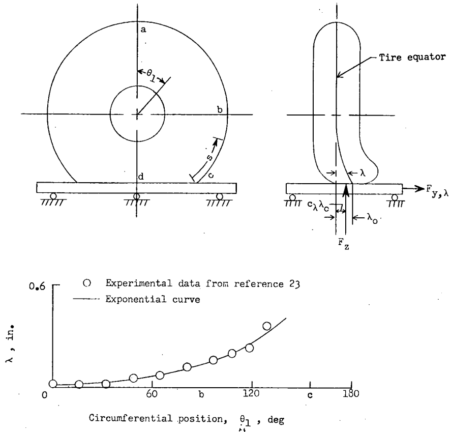
Figure 17.- Sketch illustrating tire lateral distortion for combined vertical and lateral loading.
