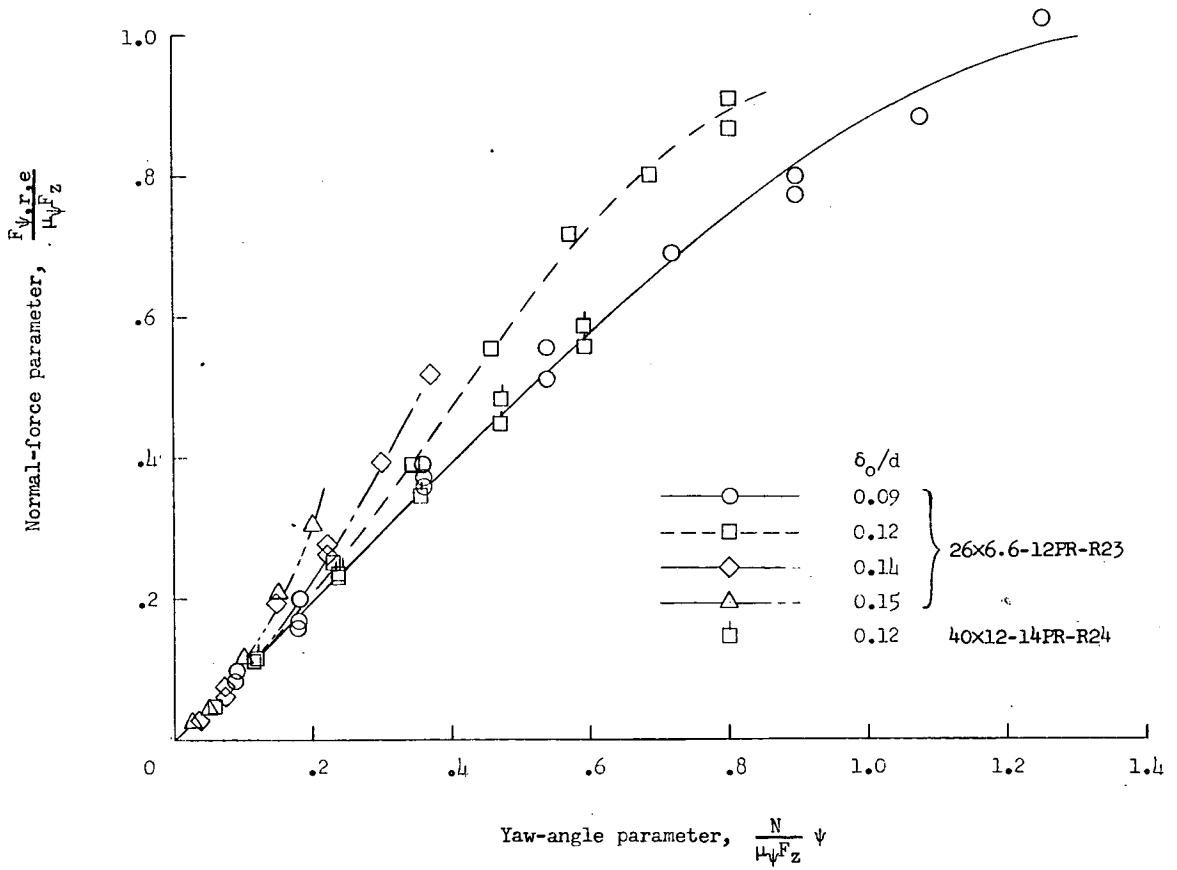
Figure 47.- Variation of steady-state normal force with yaw angle for large vertical deflections.
