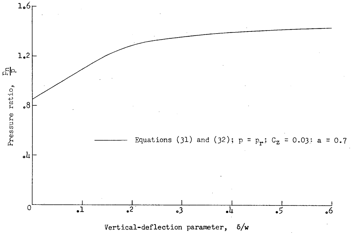
Figure 16.- Variation with vertical-deflection parameter of ratio of net footprint pressure to inflation pressure.
