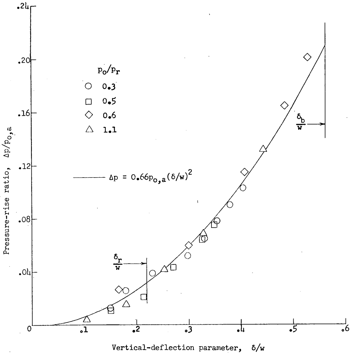
Figure 8.- Variation of pressure-rise ratio \Delta p/p_{0,a} with vertical-deflection parameter for a 28x9-10PR-I(27-inch)R21-E2 tire.
