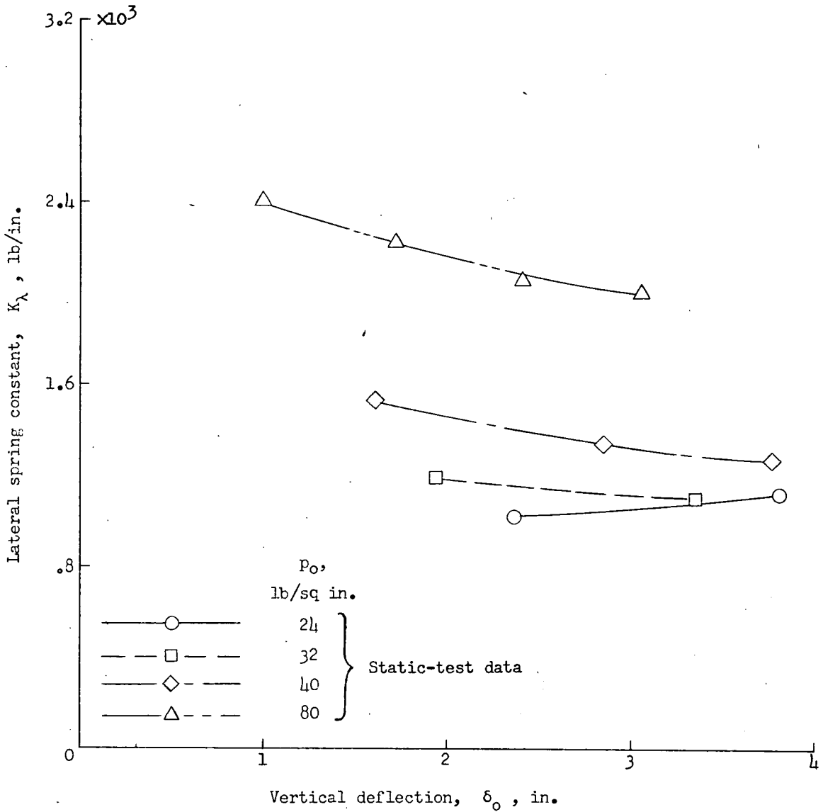
Figure 18.- Variation of lateral spring constant with vertical deflection and inflation pressure for a 28x9-10PR-I(27-inch)-R21-E2 tire.
