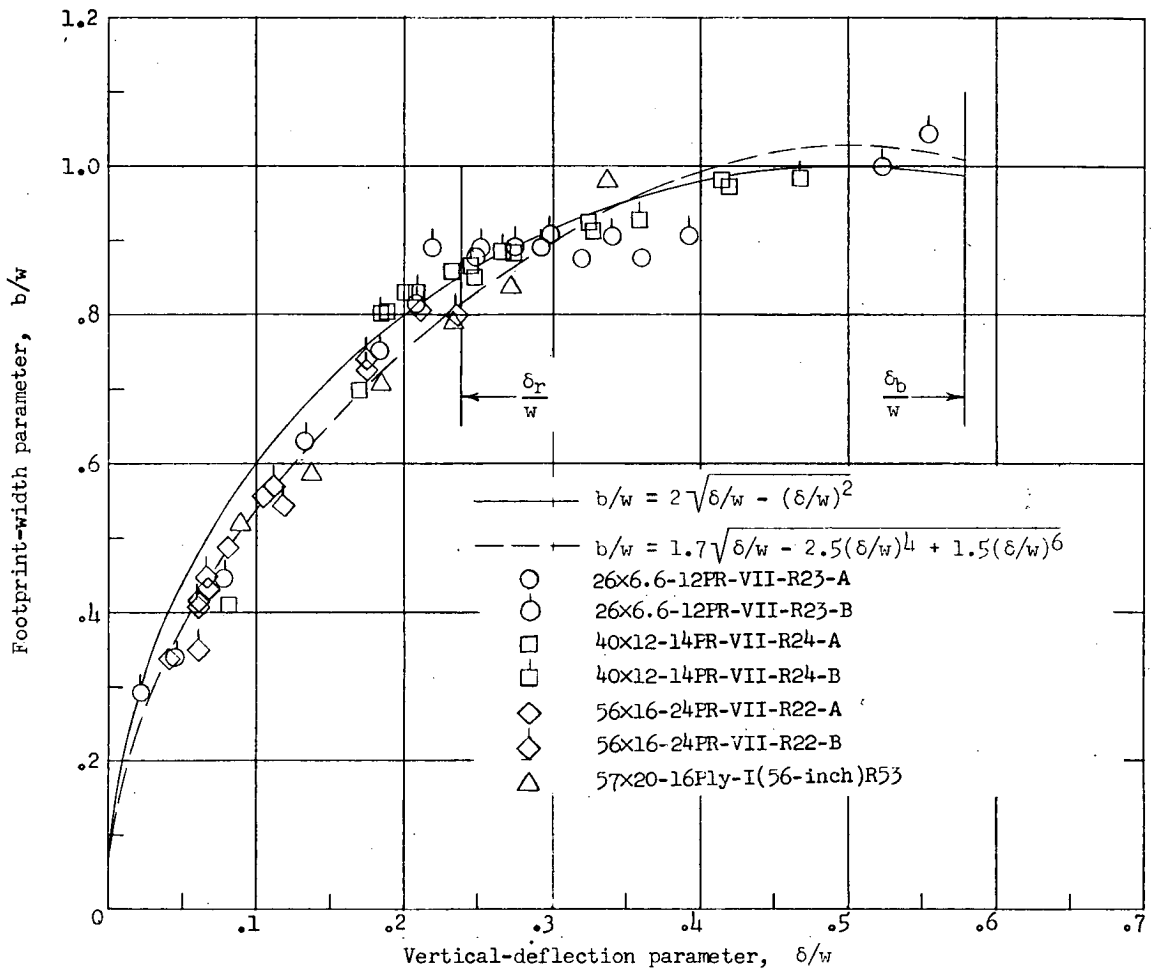
Figure 5.- Variation of footprint-width parameter with vertical-deflection parameter.
