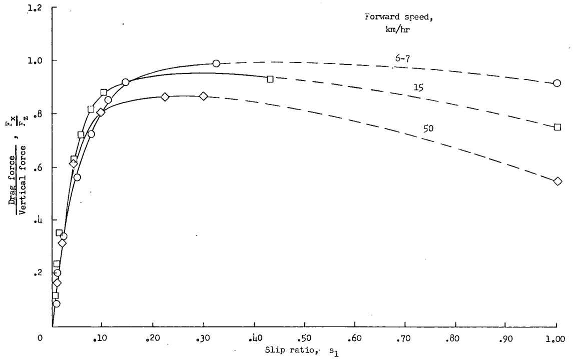
Figure 53.- Experimental variation of drag force with slip ratio for braking tests of an automobile tire on dry concrete. (Data from ref. 13.)
