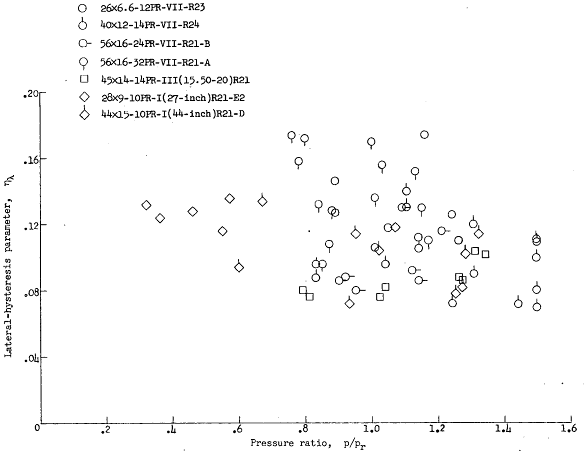
Figure 63.- Variation of static lateral-hysteresis parameter with inflation pressure for several types I, III, and VII tires.
