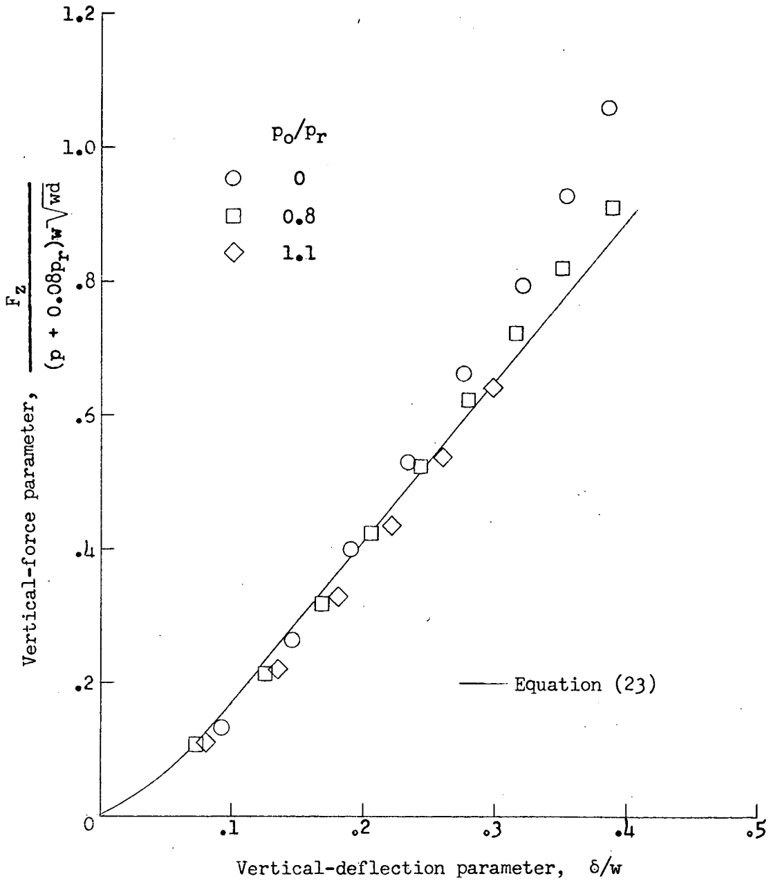
Figure 12.- Variation of vertical-force parameter with vertical-deflection parameter for a 56x16-32PR-VII-R21-A tire at several inflation pressures.
