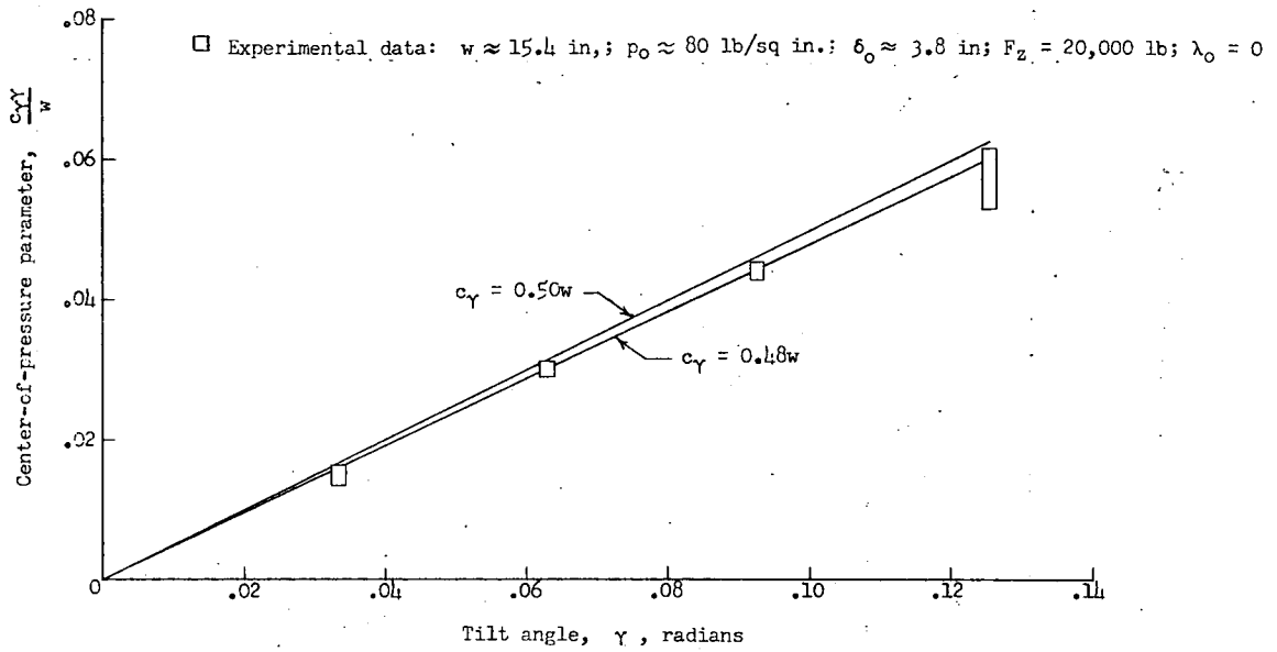
Figure 37.- Variation of vertical-force center-of-pressure parameter with tilt angle for a standing tire. (Unpublished experimental data for 45x15-14PR-III(15.50-20) tire of ref. 21.) Vertical height of test symbols indicates probable error for respective test points.
