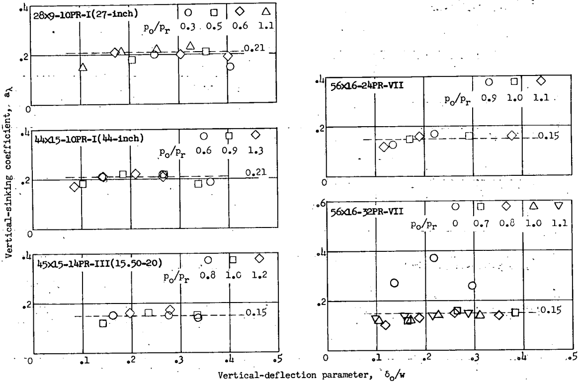
Figure 23.- Variation of vertical-sinking coefficient with vertical-deflection parameter for types I, III, and VII tires. (Experimental data from ref. 21.)
