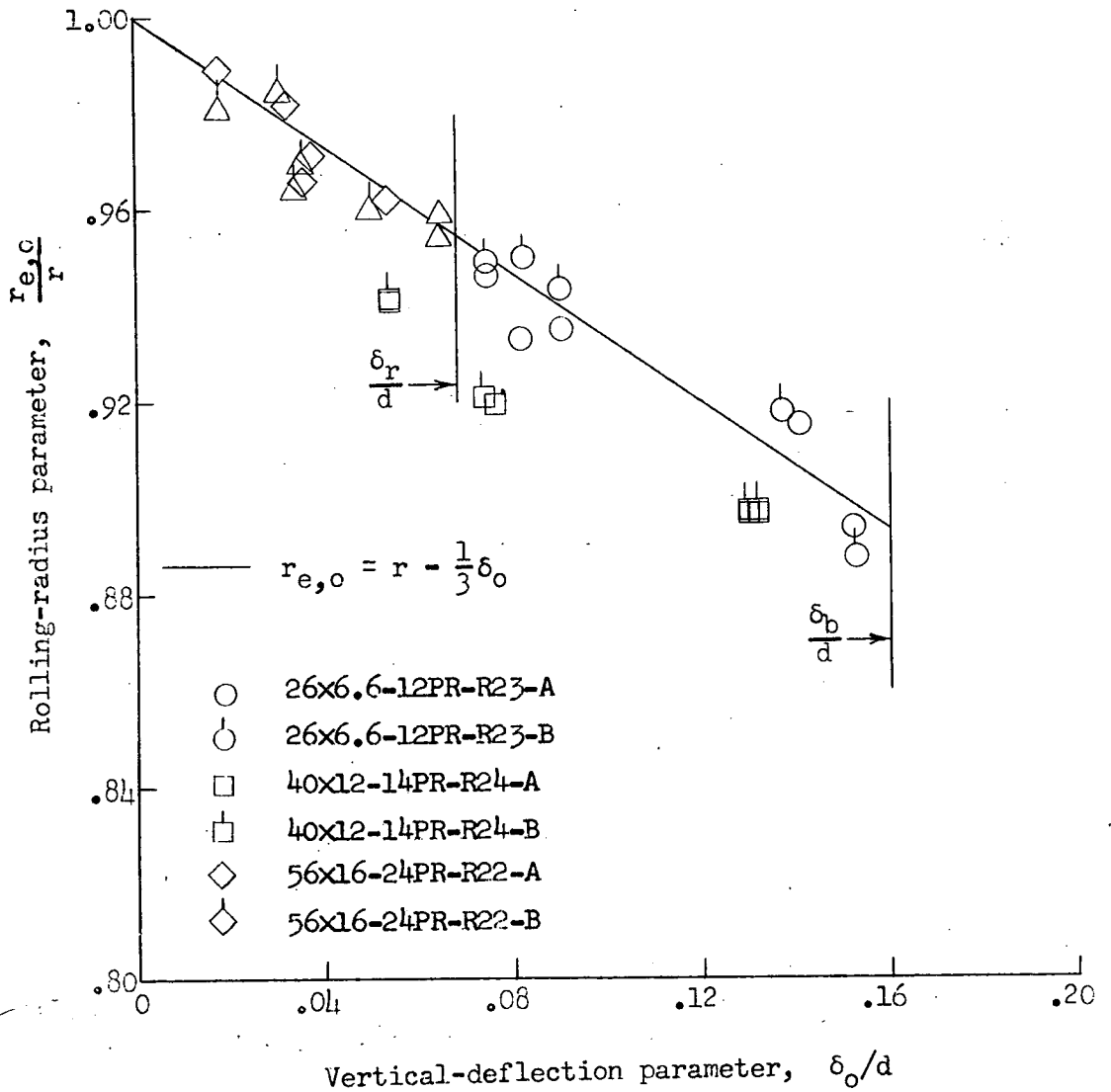
Figure 40.- Variation of rolling radius with vertical-deflection parameter for six type VII tires at very small or zero yaw angles.
