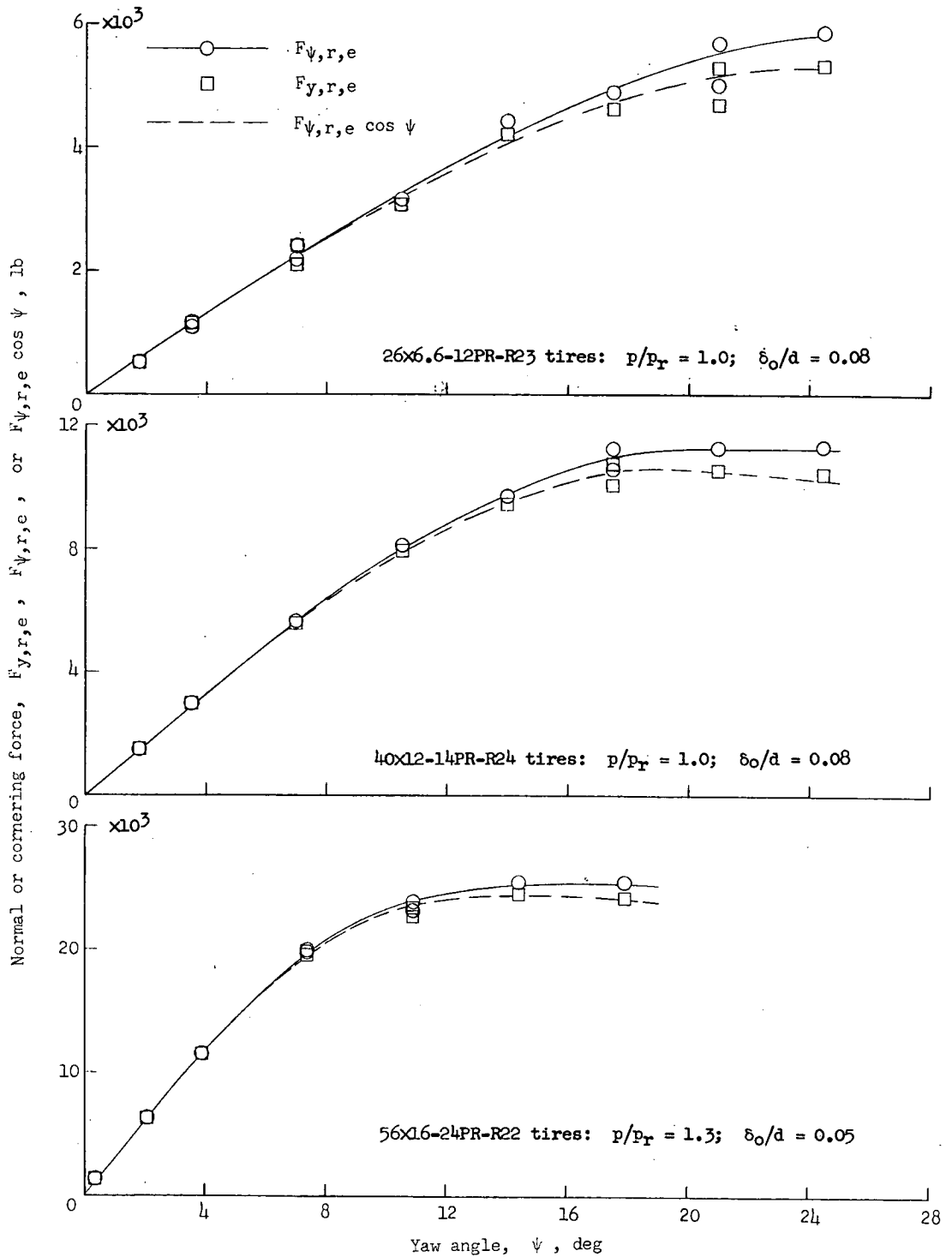
Figure 45.- Comparison of normal and cornering forces for yawed rolling of several type VII tires.
