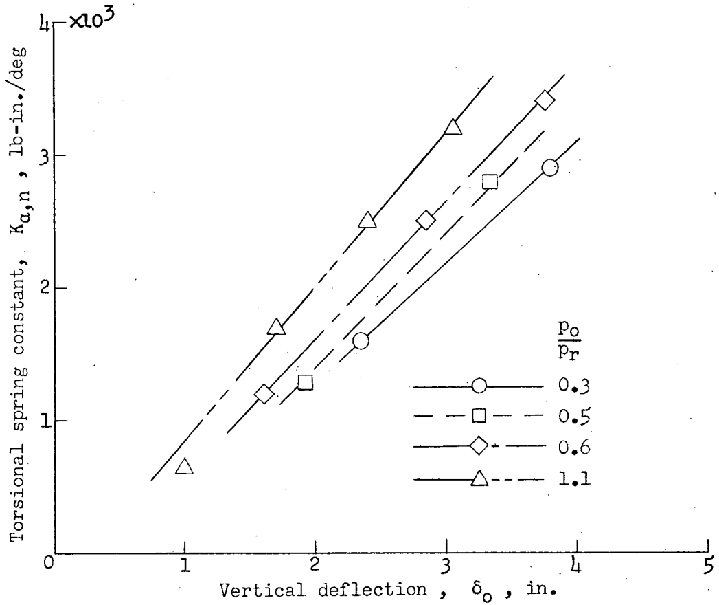
Figure 28.- Experimental variation of static torsional spring constant with vertical deflection and inflation pressure for a 28x9-10PR-I(27-inch)R21-E2 tire.
