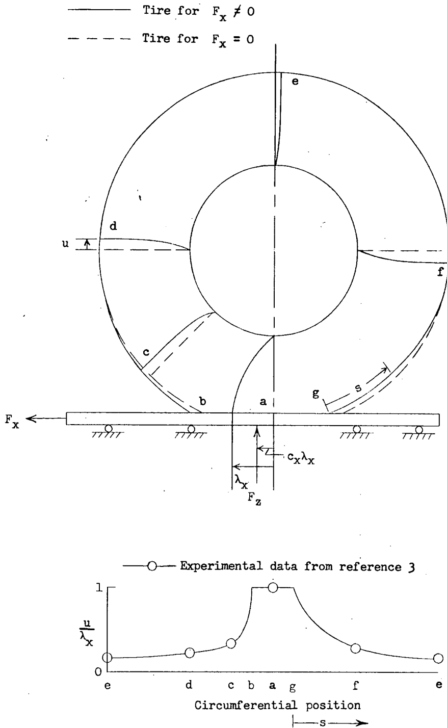
Figure 30.- Sketch illustrating tire distortion for combined vertical and fore-and-aft loading.
