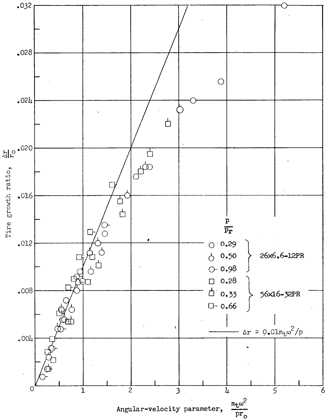
Figure 60.- Growth of tire radius due to centrifugal forces for two type VII tires. (Experimental data from tables III and IV.)
