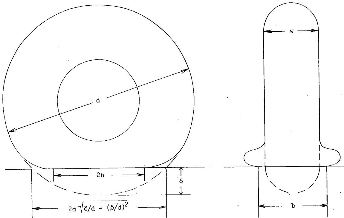
Figure 2.- Sketch of tire under pure vertical loading.
