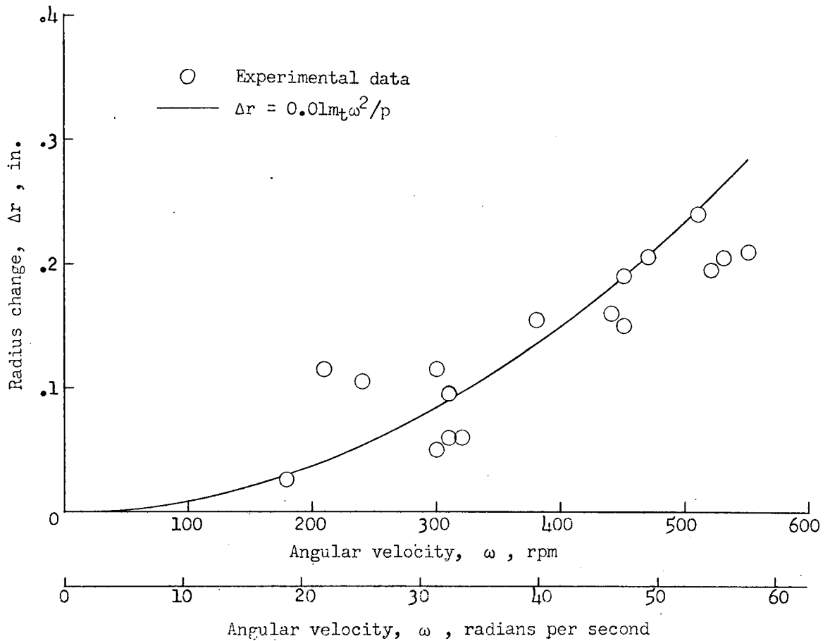
Figure 61.- Growth of tire radius due to centrifugal forces for a pair of .57x20-16Ply-I(56-inch)R53 tires. r = 28.3 inches; p = 80 pounds per square inch; m_t (estimated) = 8.2 slugs.
