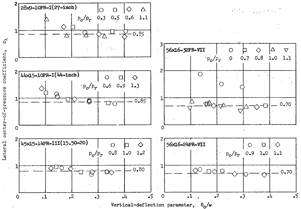
Figure 22.- Variation of lateral center-of-pressure coefficient with vertical-deflection parameter for types I, III, and VII tires. (Experimental data from ref. 21.)
