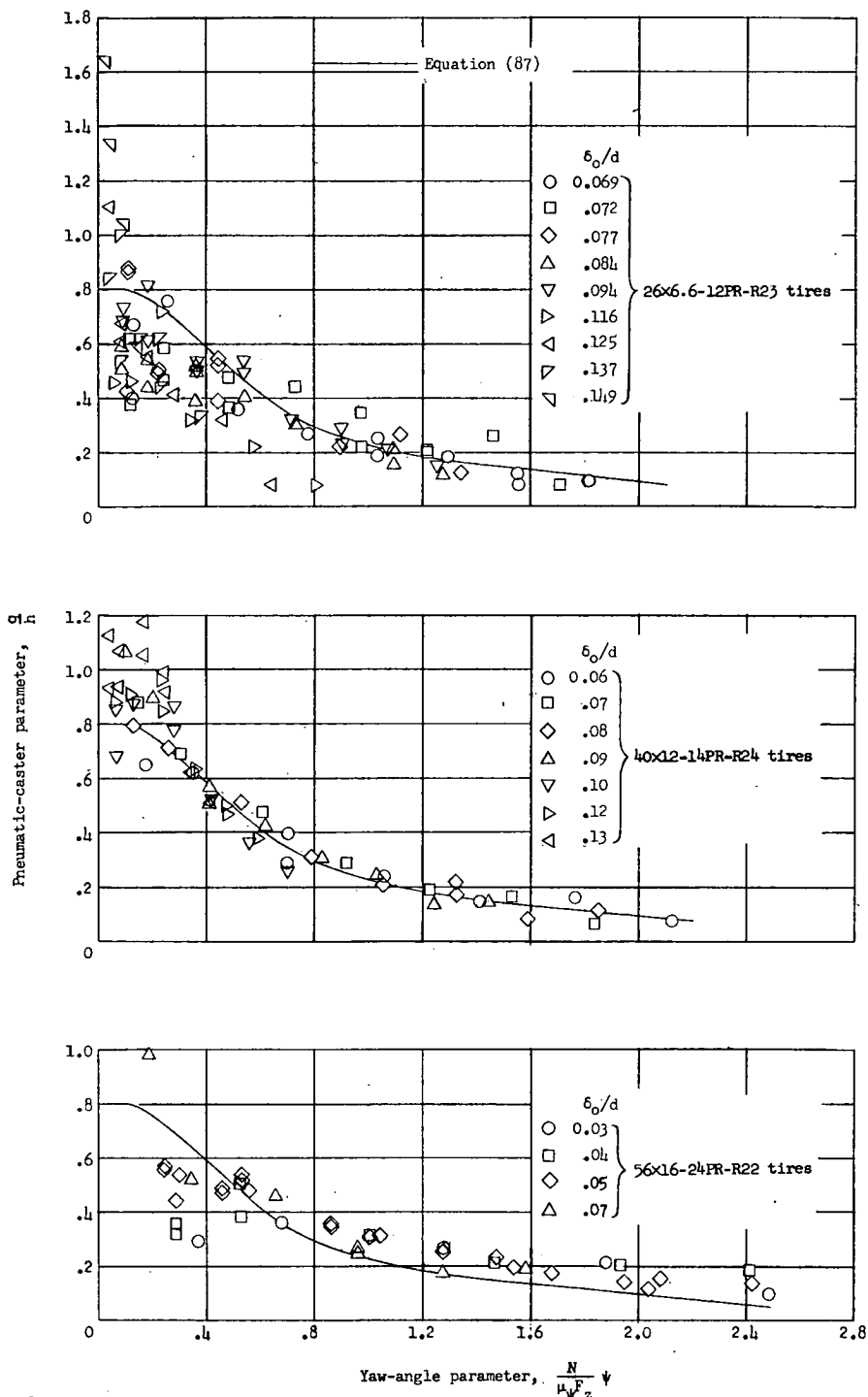
Figure 51.- Variation of pneumatic-caster parameter with yaw-angle parameter for several pairs of type VII tires.
