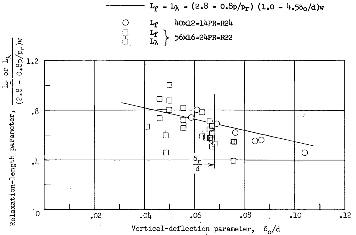
Figure 38.- Variation of unyawed-rolling relaxation-length parameters with vertical-deflection parameter for two pairs of type VII tires.
