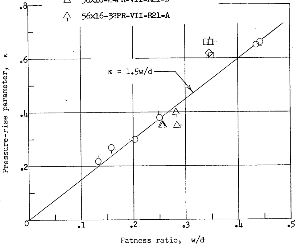
Figure 9.- Variation of pressure-rise parameter \kappa with tire fatness ratio.
