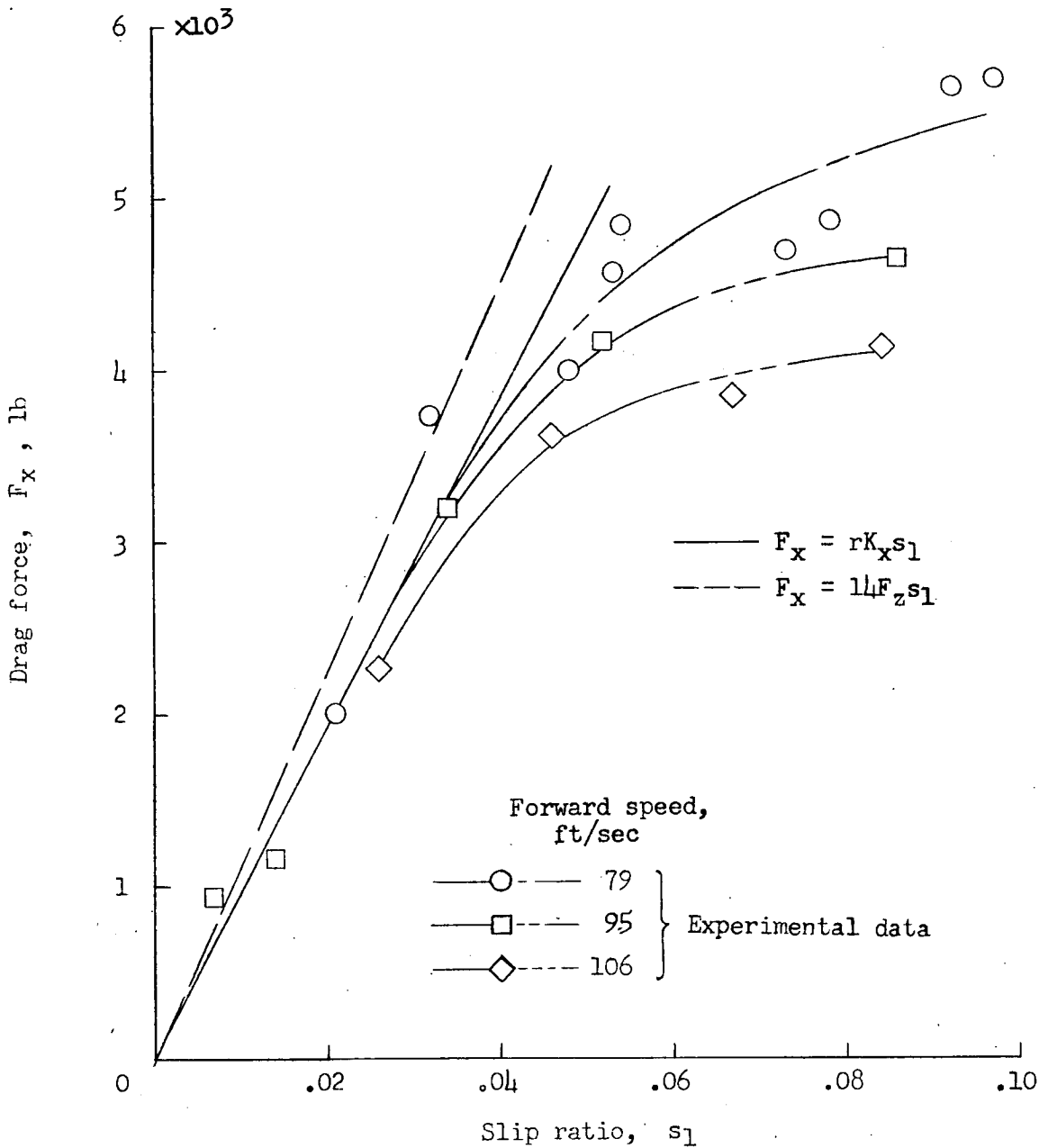
Figure 54.- Variation of drag force with slip ratio for braking tests of a 48x17-16PR-III(17.00-20)RU aircraft tire. F_z \approx 8,000 pounds; K_x (estimated) \approx 4,000 pounds per inch.
