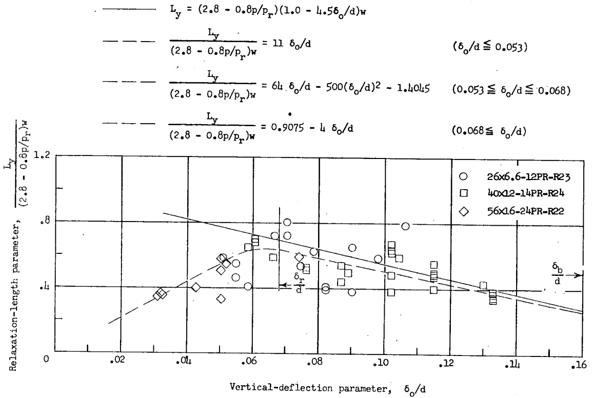
Figure 39.- Variation of yawed-rolling relaxation-length parameter with vertical-deflection parameter for three type VII tires.
