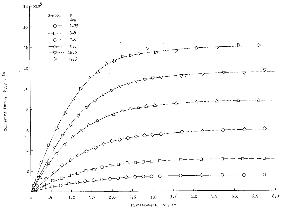
Figure 43.- Buildup of cornering force with distance rolled for a pair of 40x12-14PR-VII-R24 tires. p/p_r = 1.5 ; \delta_0/d = 0.10 .
