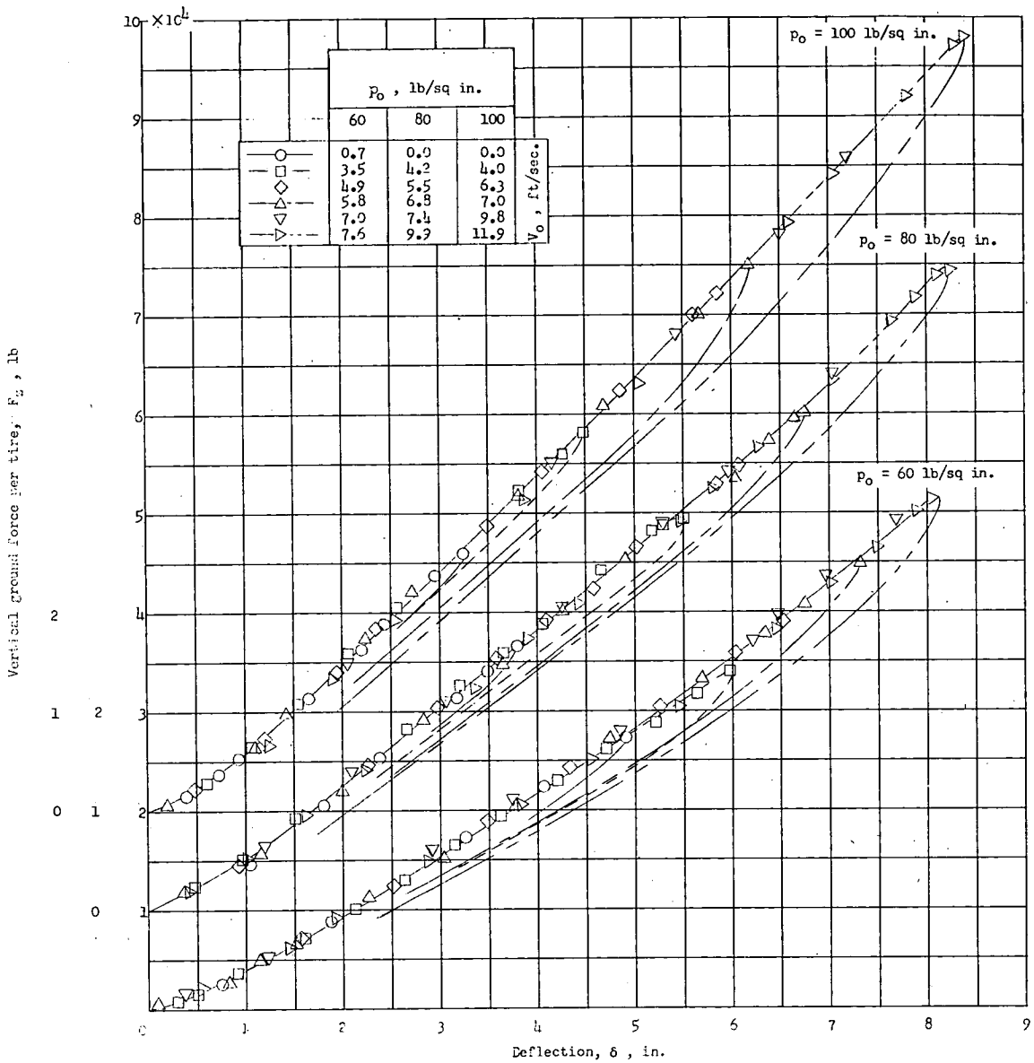
Figure 14.- Variations of vertical ground force, with vertical tire deflection obtained from drop tests without prerotation for pair of 57x20-16Ply-I(56-inch)R53 tires.
