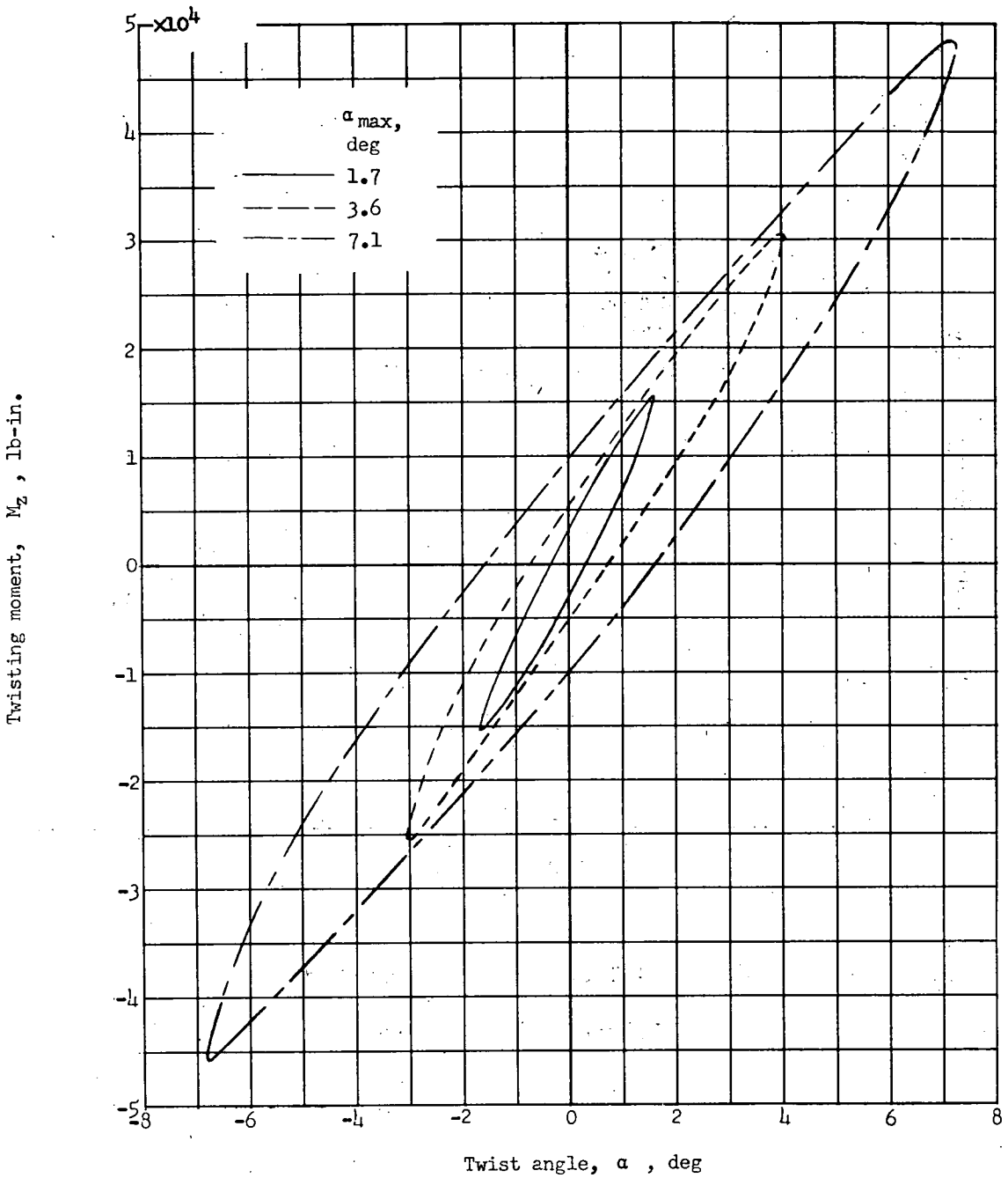
Figure 26.- Variation of twisting moment with twist angle for a 40 \times 12-14PR-VII-R24-B tire for several different amplitudes. p/p_r = 1.5 ; \delta_0/d = 0.10 .
