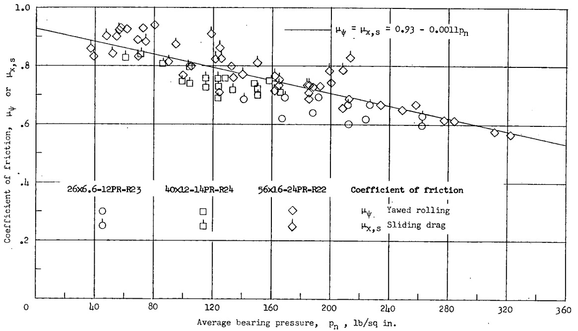
Figure 52.- Variation of sliding-drag and yawed-rolling coefficients of friction with bearing pressure from slow-speed tests of several type VII tires.
