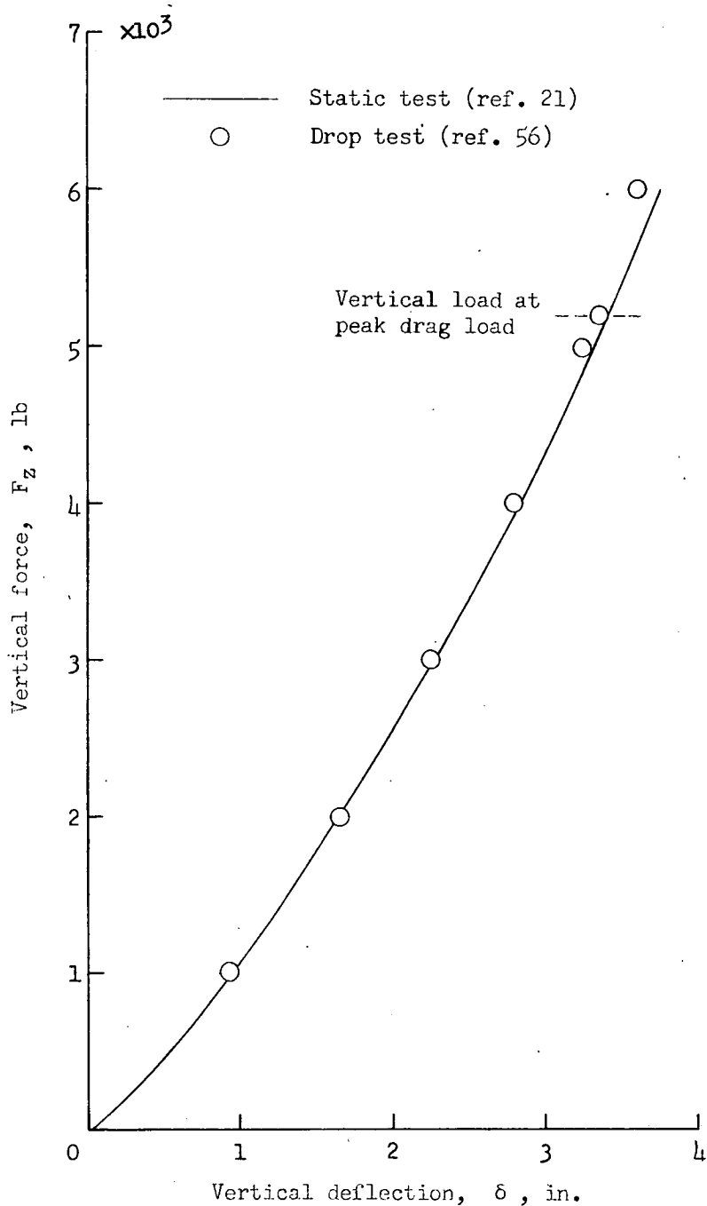
Figure 59.- Comparison of static vertical-force-deflection curve with force-deflection curve obtained from prerotation drop tests with initial peripheral velocity of 88 feet per second and initial vertical velocity of 7.5 feet per second. Data for 28x9-10PR-I(27-inch) tires; p_0 = 32 pounds per square inch.
