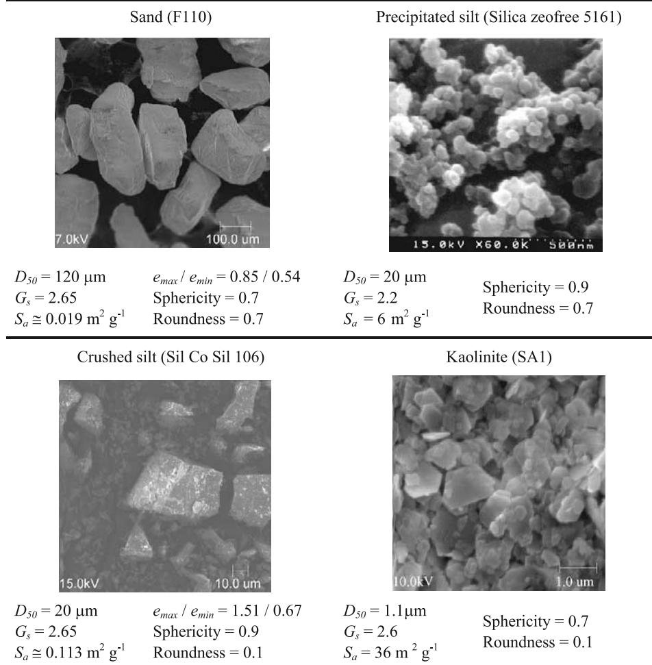
Figure 1. Characteristics of tested soils, compiled from Santamarina and Cho [2001], Klein [1999], Parks [1990], and Guimaraes [2001]. Specific surface for kaolinite and precipitated silt was measured using methylene blue (wet method). SEM pictures were provided by A. Palomino.
