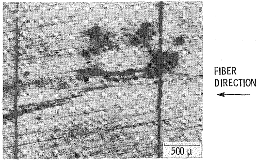
Figure 4. - A typical 3-point bend specimen stressed above the non-linear range showing matrix cracks normal to fibers on the tensile surface.
