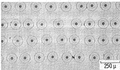
Figure 2. - A typical cross section of SiC/RBSN composite showing fiber distribution.
