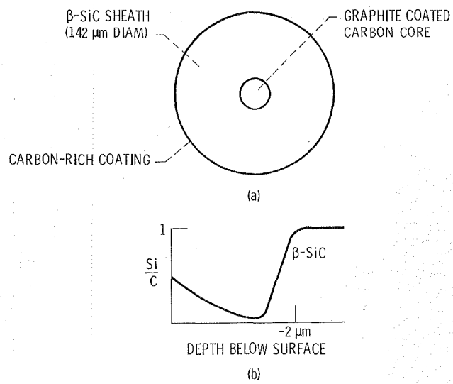
Figure 1. (a) Schematic of cross section of CVD SiC fiber. (b) The composition profile of carbon-rich coating on the surface of SiC fiber (AVCO SCS-6 fiber).
