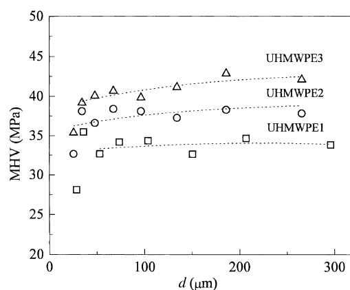
Figure 4. Dependence of Vickers microhardness as a function of diagonals of the indentation.
