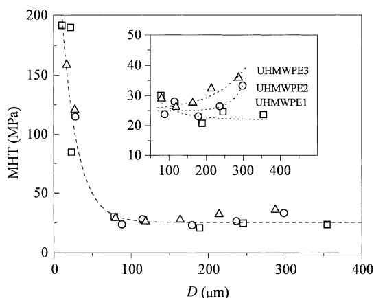
Figure 5. Dependence of Total microhardness as a function of diagonals of the indentations in the loaded state (the inset shows the same dependence for high values of the diagonal).
