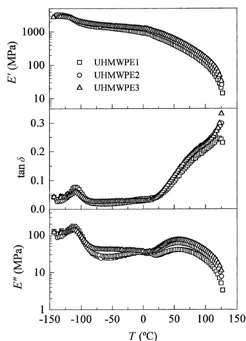
Figure 3. Comparison of the temperature dependences of E' , E'' and \tan \delta as a function of the temperature, measured at 3 Hz, for the three samples studied.
