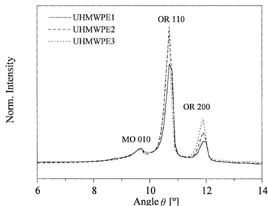
Figure 1. Wide-angle X-Ray diffraction patterns of UHMWPE samples. The diffractograms were normalized to the same total intensity.
