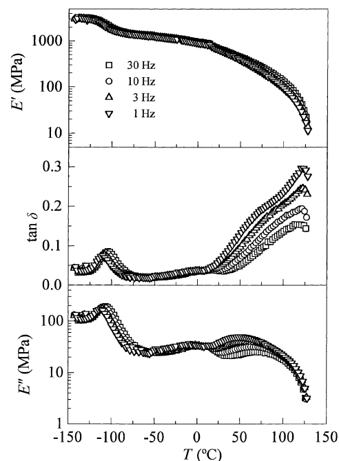
Figure 2. Temperature dependences of E' , E'' and \tan \delta for UHMWPE sample 1 measured at the frequencies indicated.
